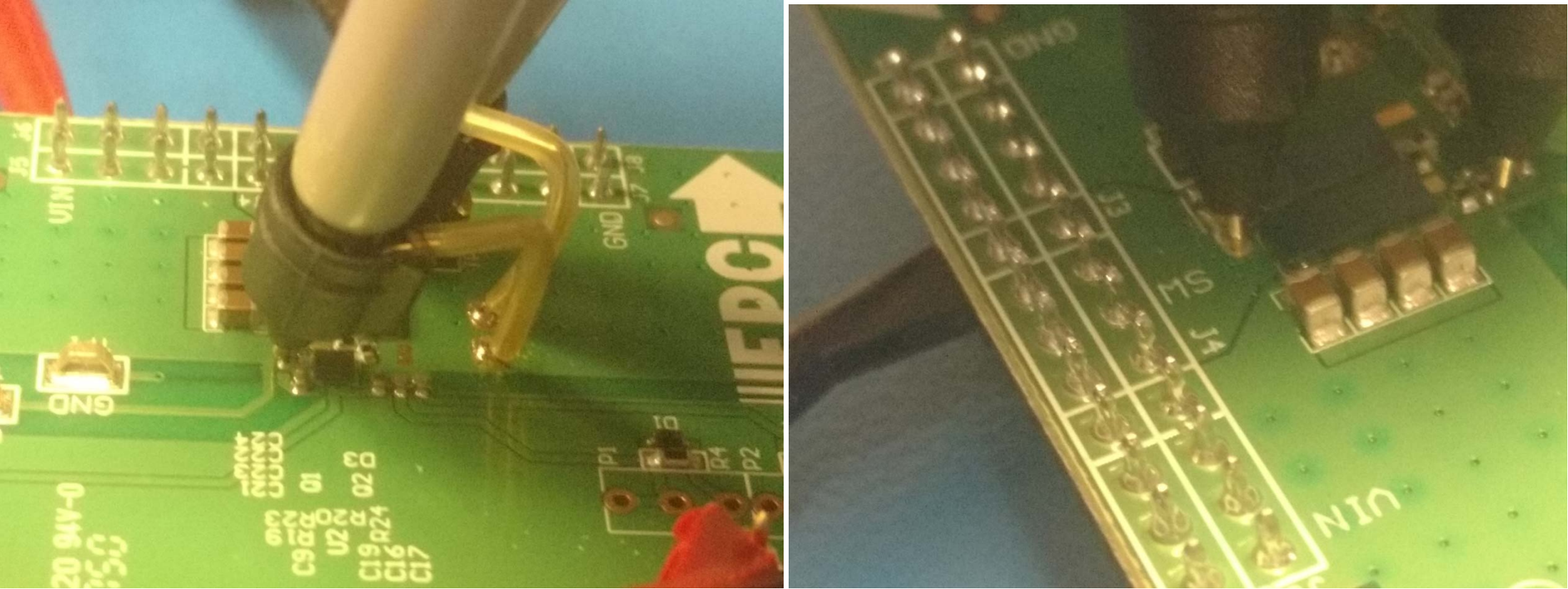
Figure 3&4 - LMGEVM_Probes
