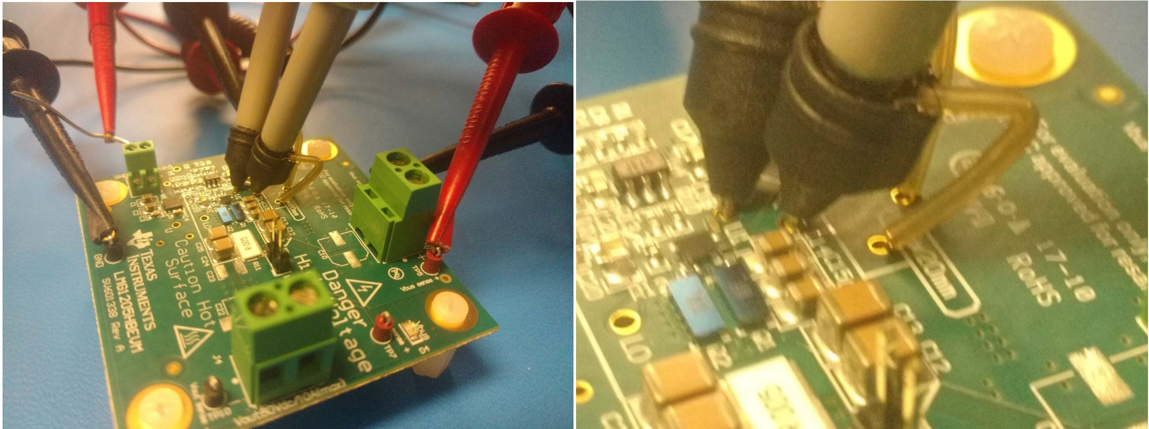
Figure 3&4 - LMGEVM_Probes
