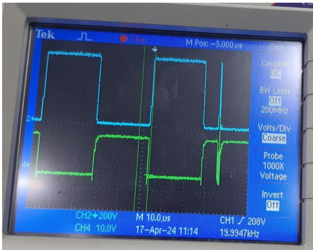
Figure 1: CH2: Voltage across device and CH4: Gate Voltage
