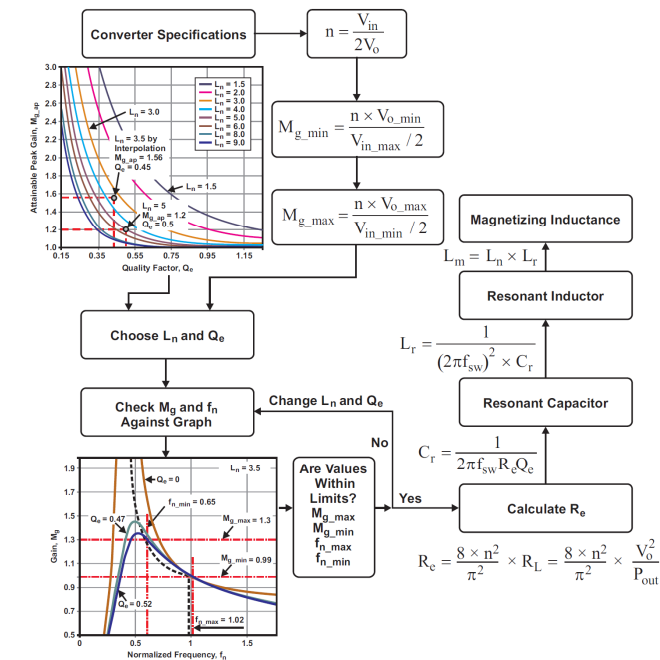
Fig. 14. Flowchart of resonant-network design.
