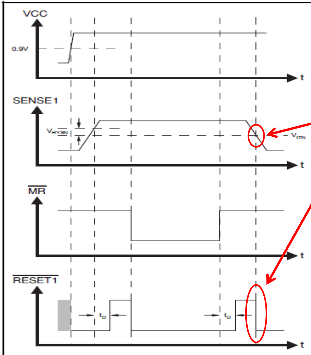
Figure 24. SVS-1 Timing Diagram
