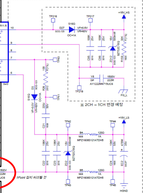
+15V / 150mA & 4CH(3+1) Digital Isolator
