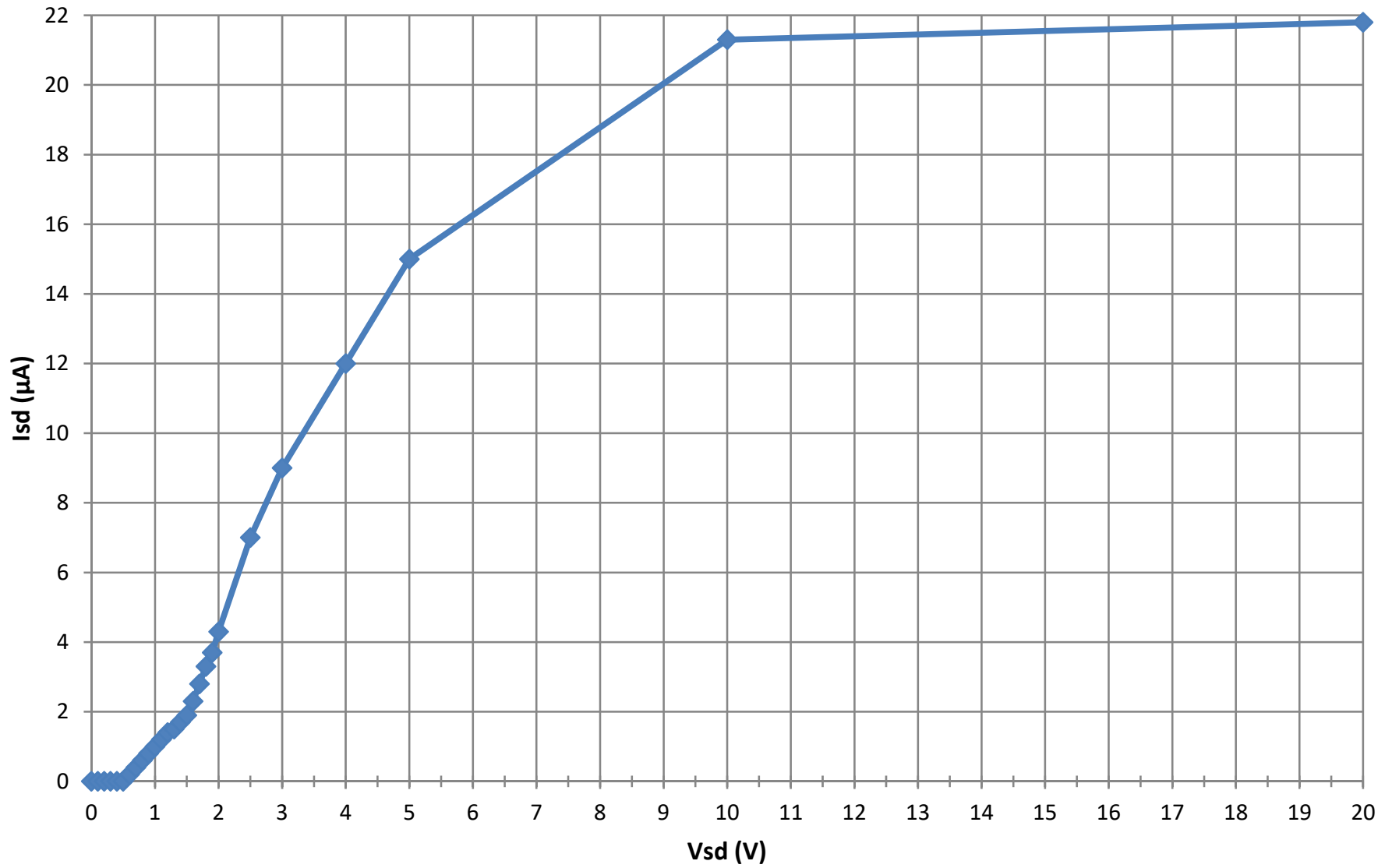
LM2936BM-5.0 Isd-vs-Vsd Vin= 12V, Iout= 1mA, Tj= 25°C
