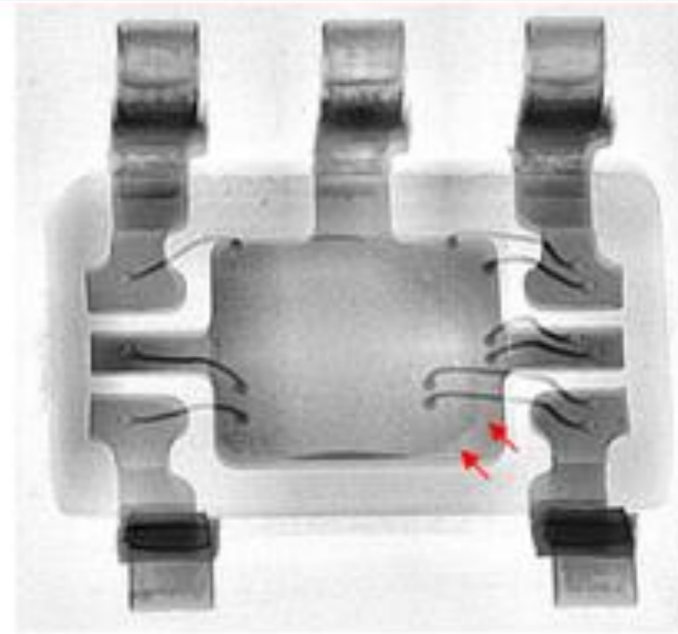
Tilt View
