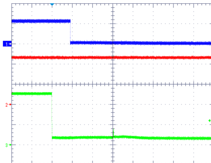
Figure 13. Output Shutdown Using UVLO Pin
