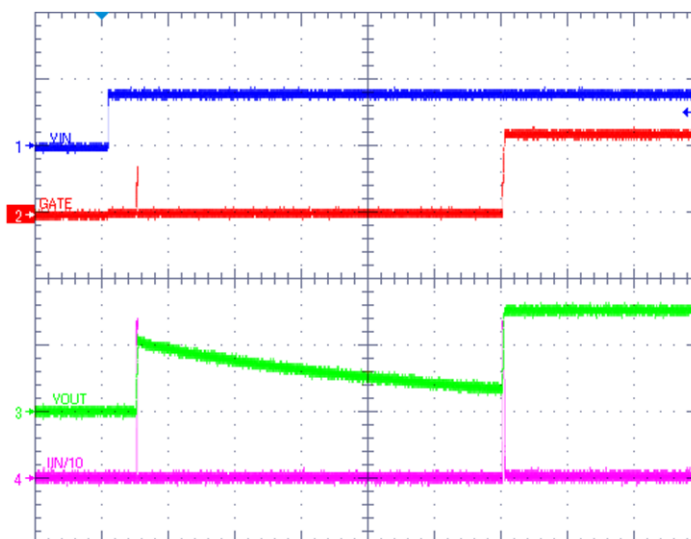
Figure 17. Inrush Current with 4900- \mu F Output Capacitor
