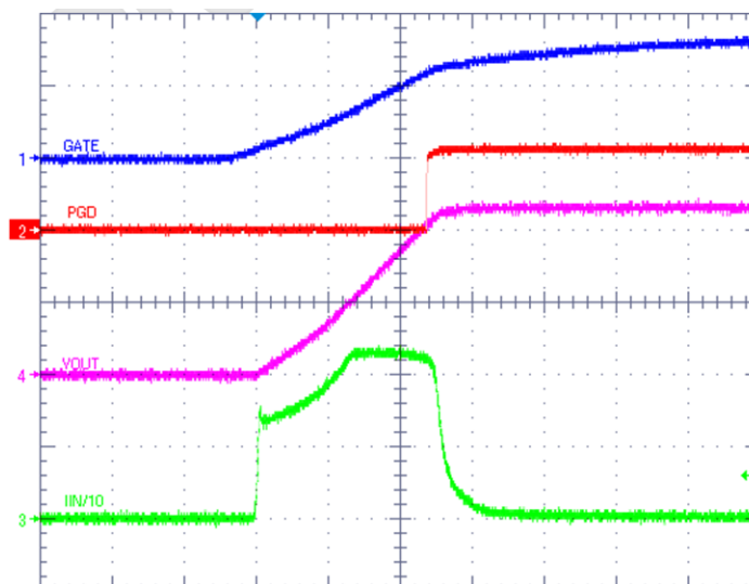
Figure 10. Turn-on Sequence with No Load Current
