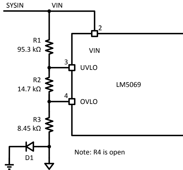
Figure 3. UVLO, OVLO Inputs (Option A)
