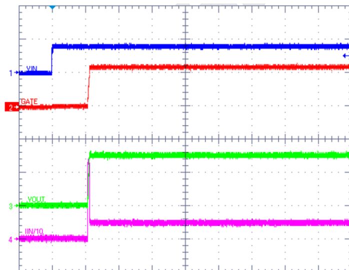
Figure 16. Inrush Current with 2550-μF Output Capacitor
