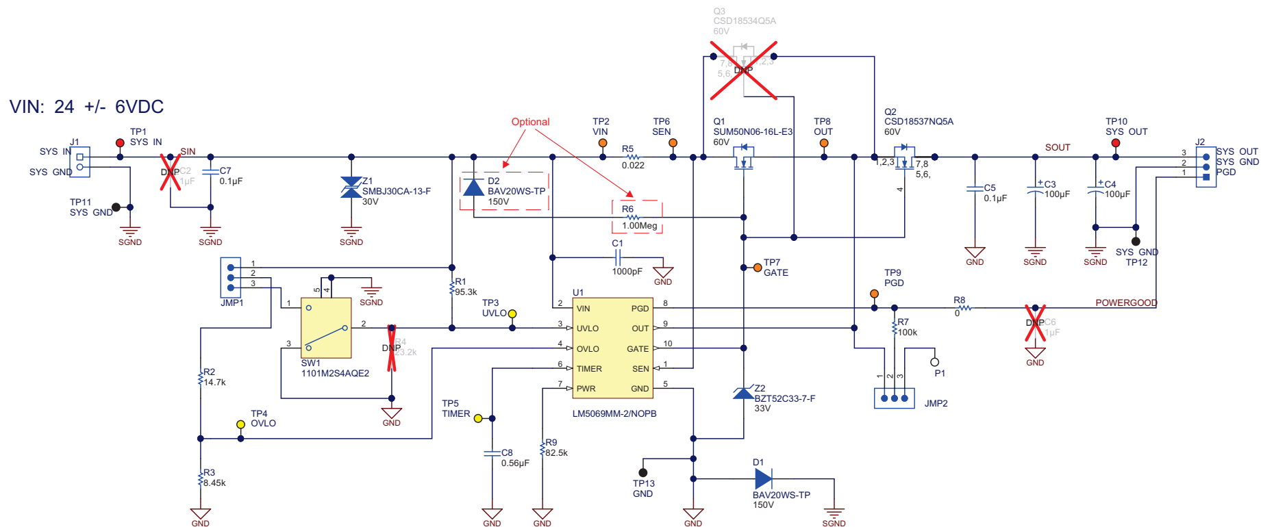
Figure 18. LM5069EVM-627 Schematic
