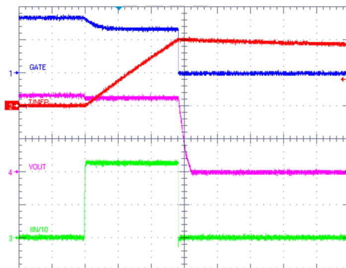
Figure 8. Fault Timeout
