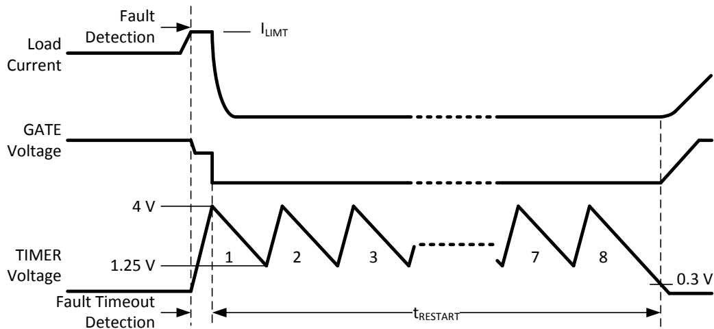
Figure 2. Fault Timeout and Restart Sequence
