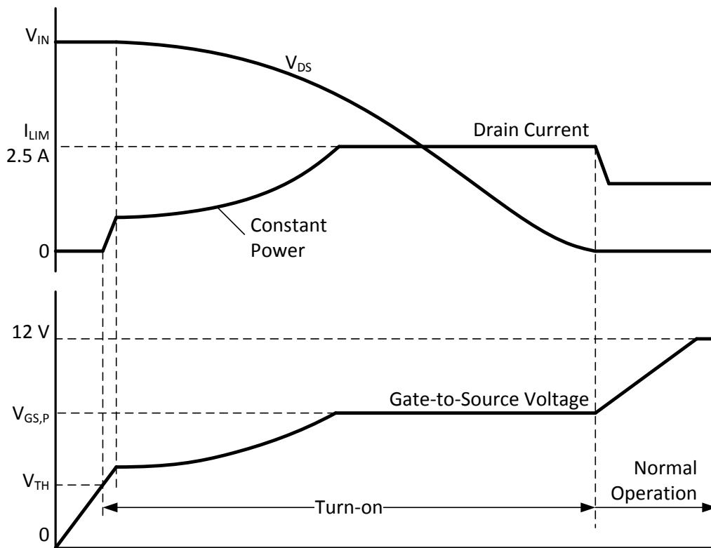
Figure 1. Power Up Using Power Limit and Current Limit
