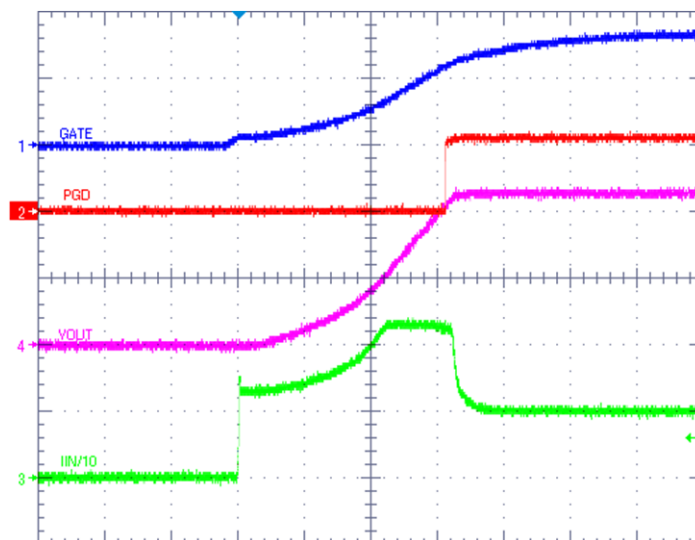
Figure 11. Turn-on Sequence with 1-A Load Current
