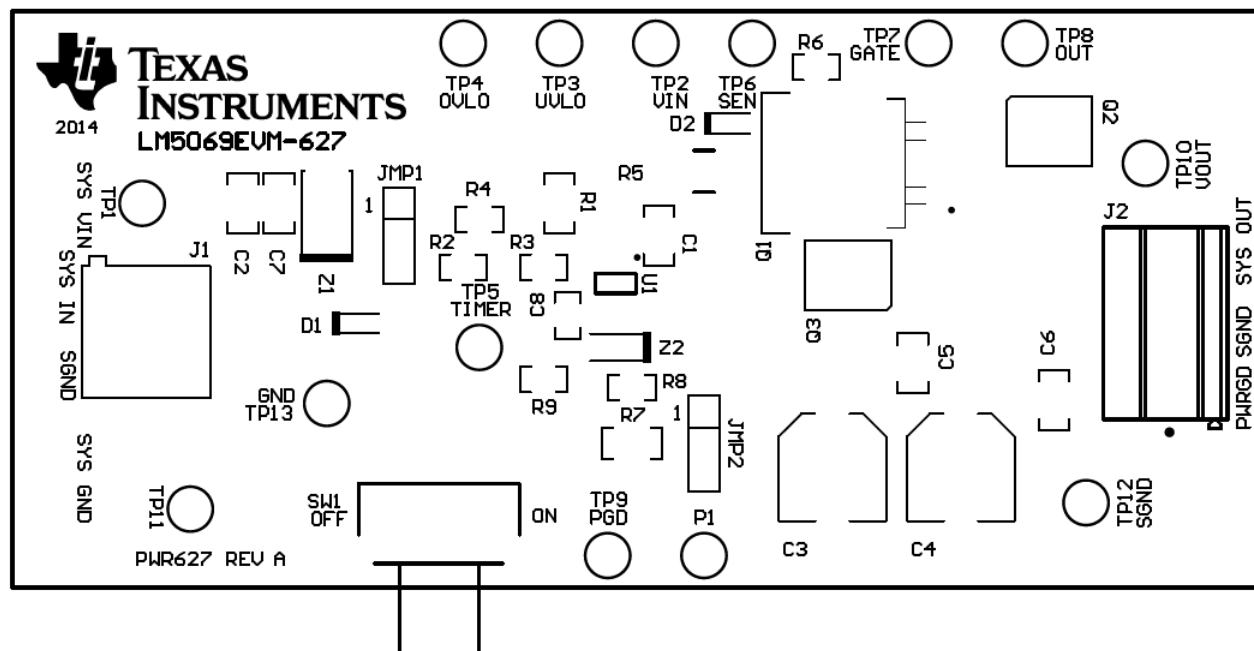
Figure 19. Top Side Placement
