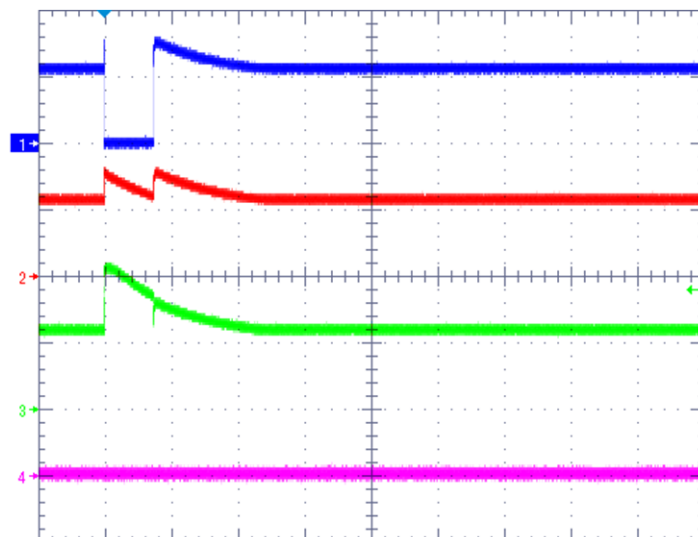
Figure 15. Input Surge (Clamped)
