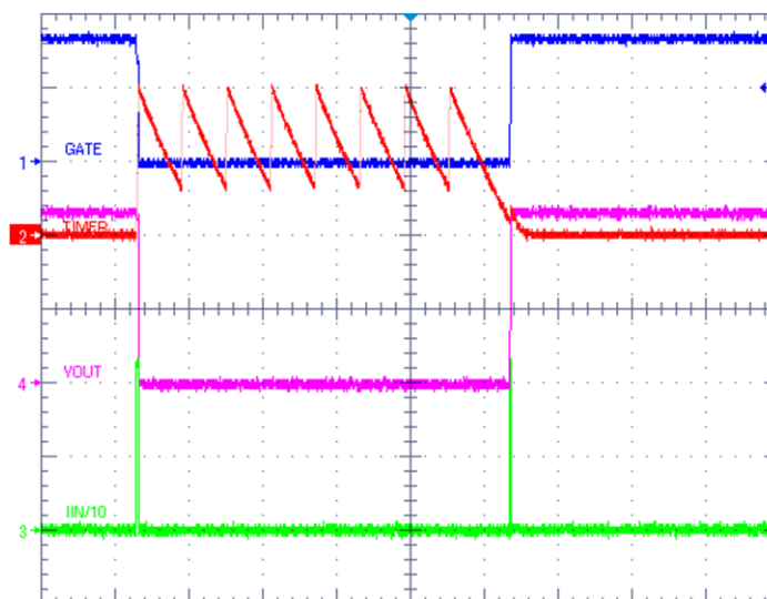
Figure 9. Restart Timing
