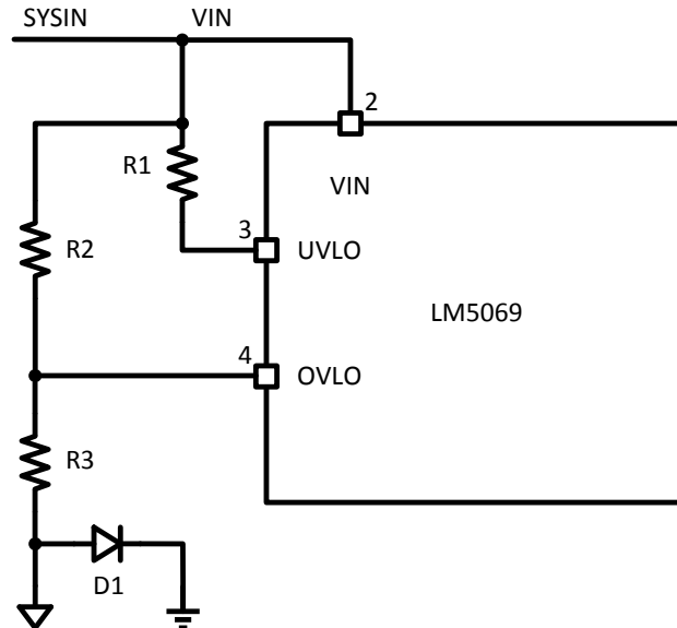
Figure 5. Minimum UVLO Threshold, Adjustable OVLO
