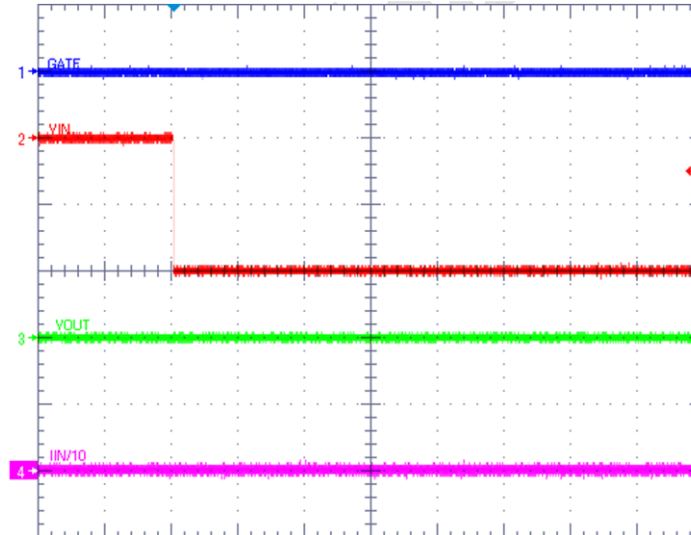
Figure 6. Reverse Polarity Input
