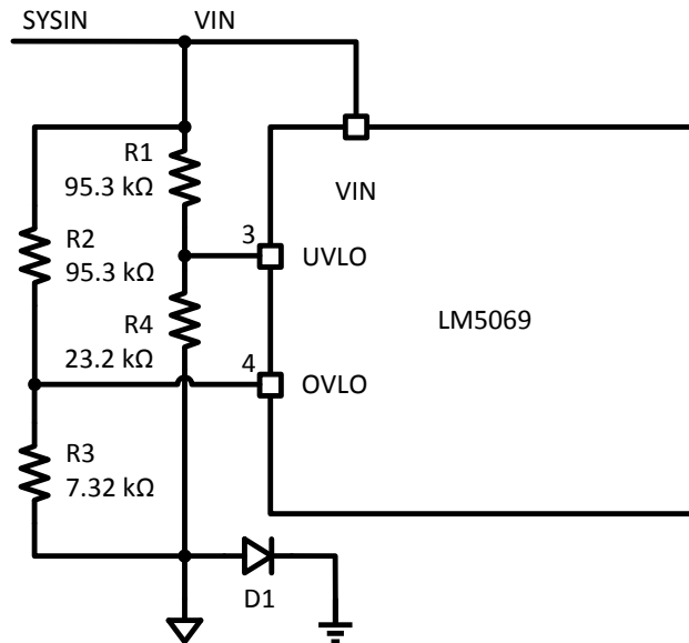
Figure 4. UVLO, OVLO Inputs (Option B)
