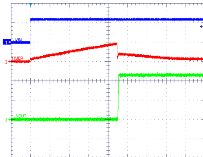
Figure 7. Insertion Timer Delay
