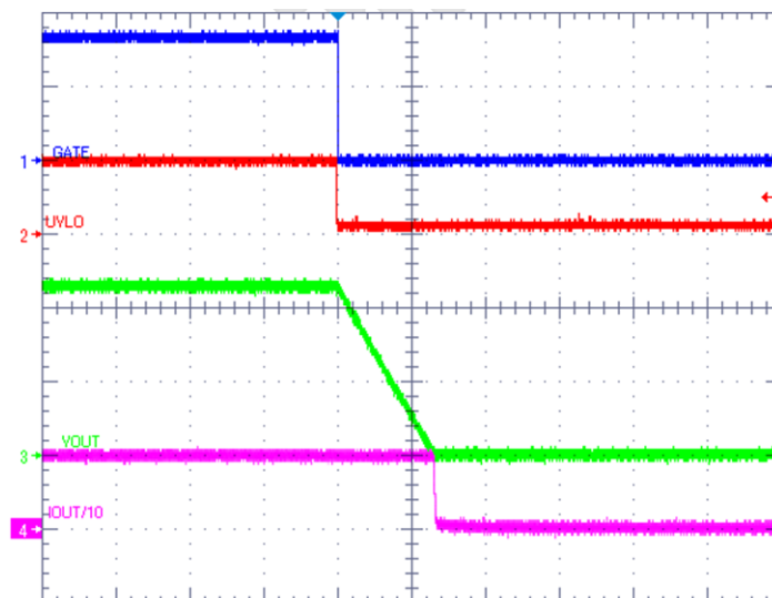
Figure 12. Output Shutdown Using UVLO Pin
