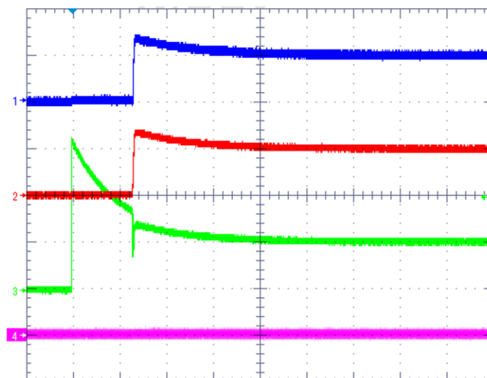
Figure 14. Input Surge (Not Clamped)
