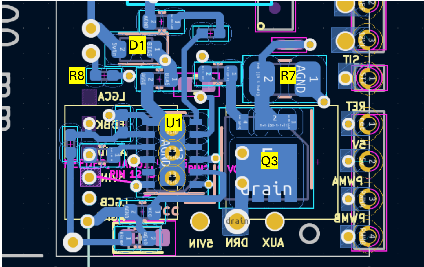
LM51561 side PCB section
