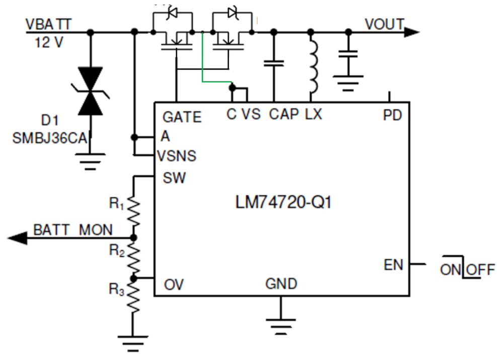
Low IQ Ideal Diode
