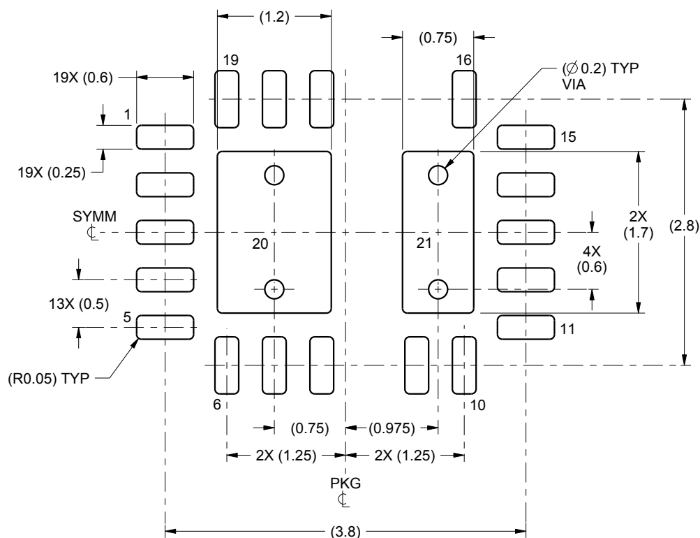
LAND PATTERN EXAMPLE SCALE:18X
