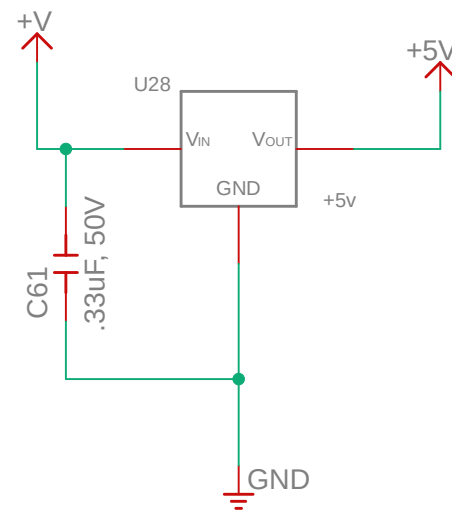
+5v Power Supply
