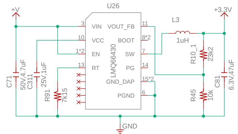
+3v3 Power Supply
