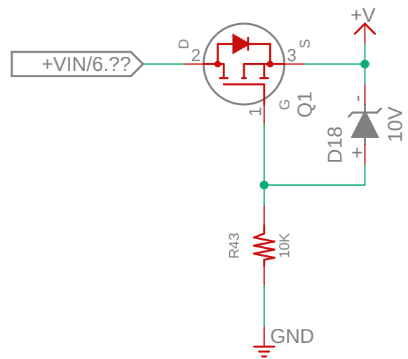
Reverse Polarity Protection
