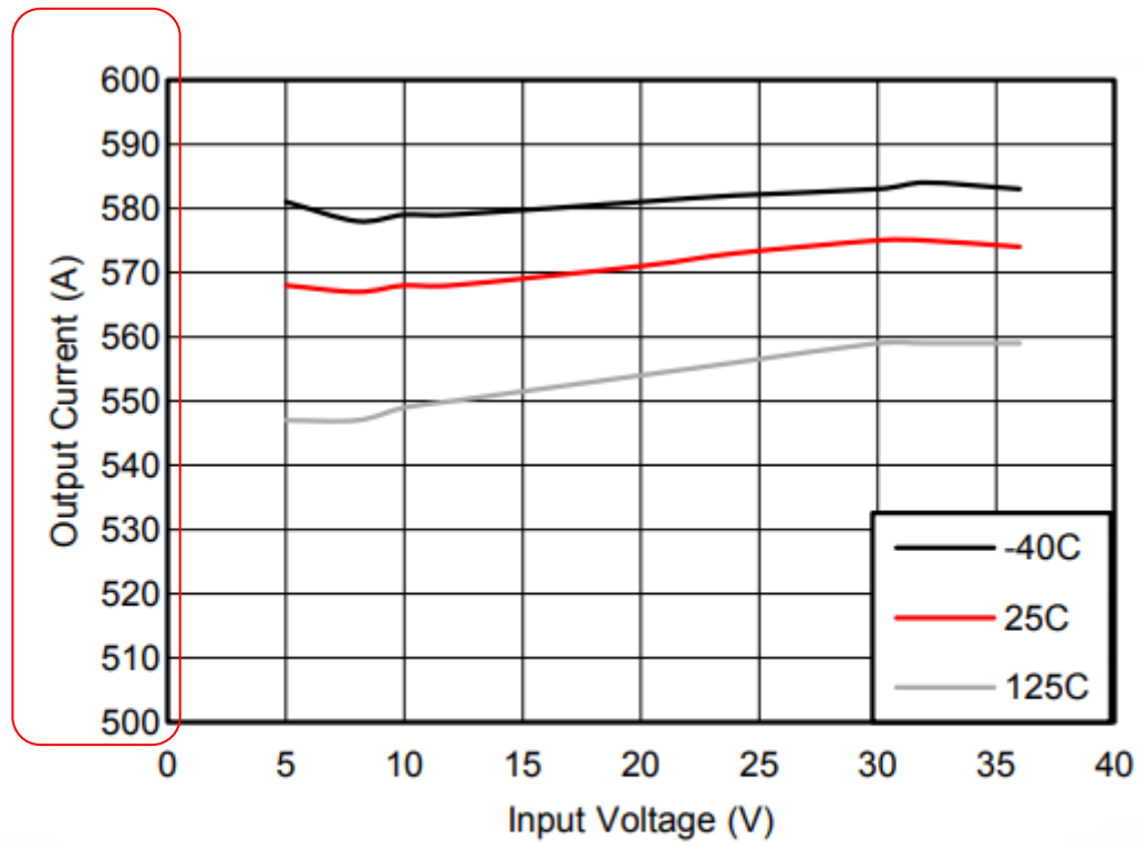
Figure 3. Short-Circuit Output Current
