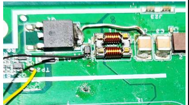
L1 Short
