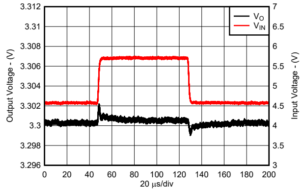
Figure 5-50. Line Transient Response for New Chip
