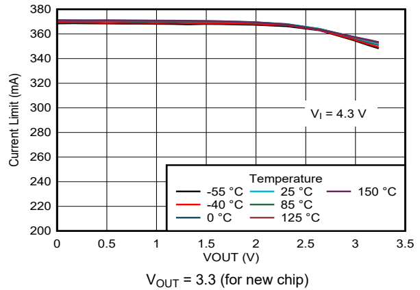
Figure 5-8. Short-Circuit Current vs Output Voltage for New Chip V_{OUT} = 3.3 (for new chip)
