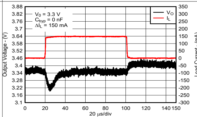
Figure 7-4. Load Transient for New Chip
