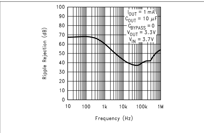
Figure 5-14. Ripple Rejection vs Frequency for Legacy Chip
