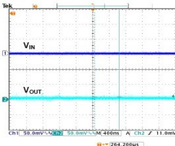
Ripple 1X Torch 150mA, V_{IN}=3.6V
