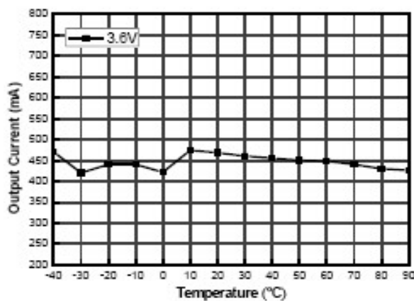
Flash Mode Output Current vs. Temperature ( C_{IN}=C_{FC}=C_{OUT}=1\mu F )
