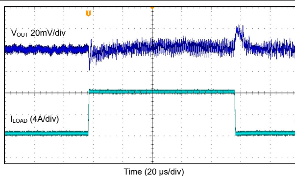
Figure 9-41. Load Transient Response, FPWM Mode. 4.4 MHz Single Phase
