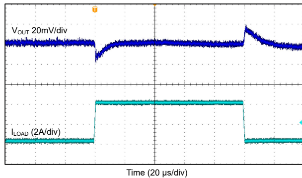
Figure 9-46. Load Transient Response, Auto Mode. 4.4 MHz 2-Phase.
