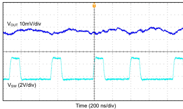
Figure 9-35. Output Voltage Ripple 2.2 MHz Single Phase. FPWM mode.
