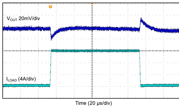
Figure 9-43. Load Transient Response, FPWM Mode. 2.2 MHz 4-Phase.
