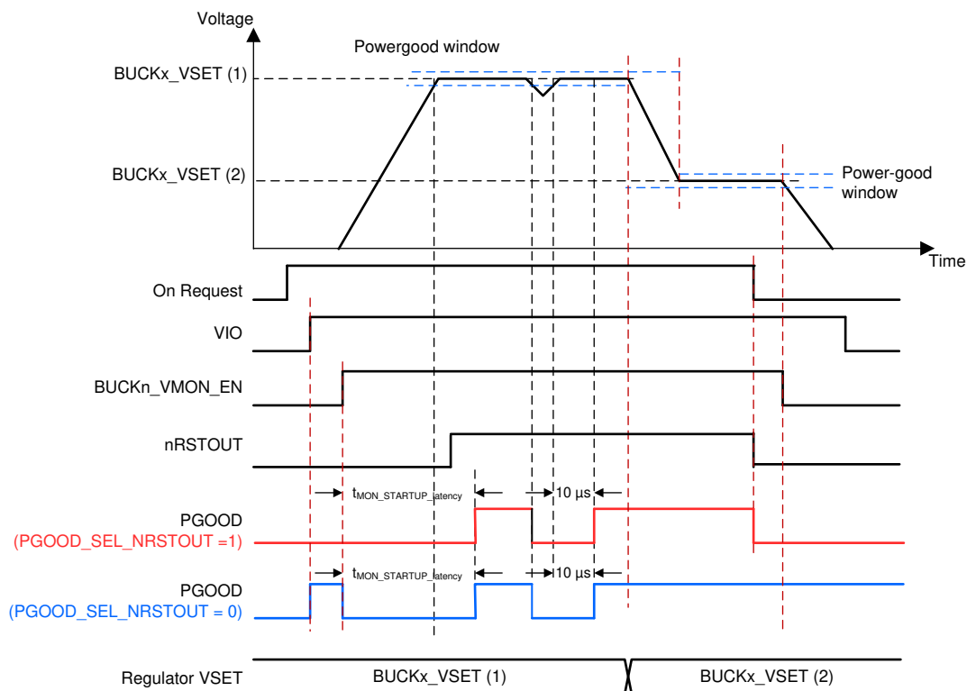
Figure 8-18. PGOOD Waveforms
