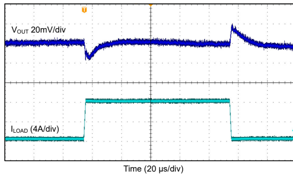
Figure 9-47. Load Transient Response, FPWM Mode. 4.4 MHz 4-Phase.
