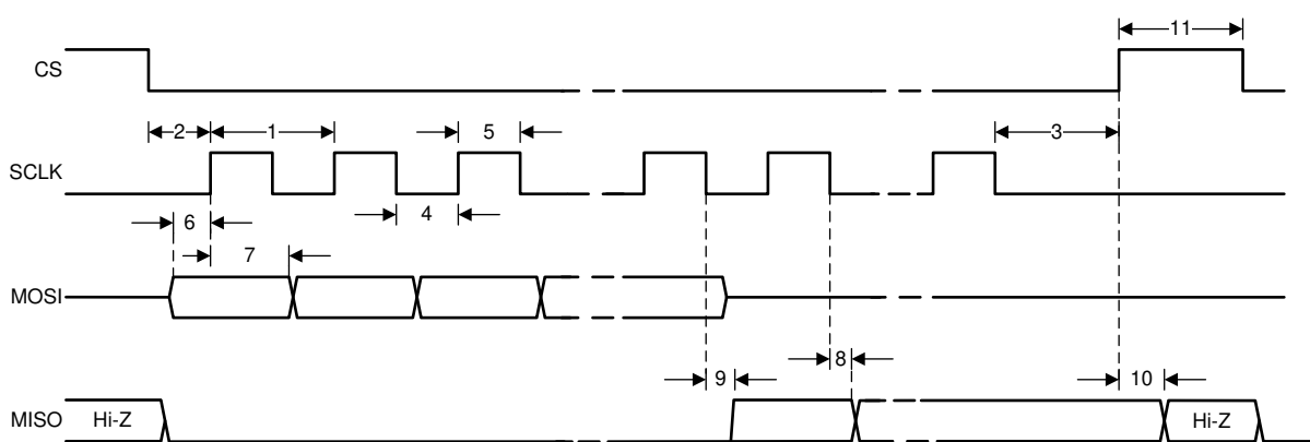
Figure 7-2. SPI Timing
