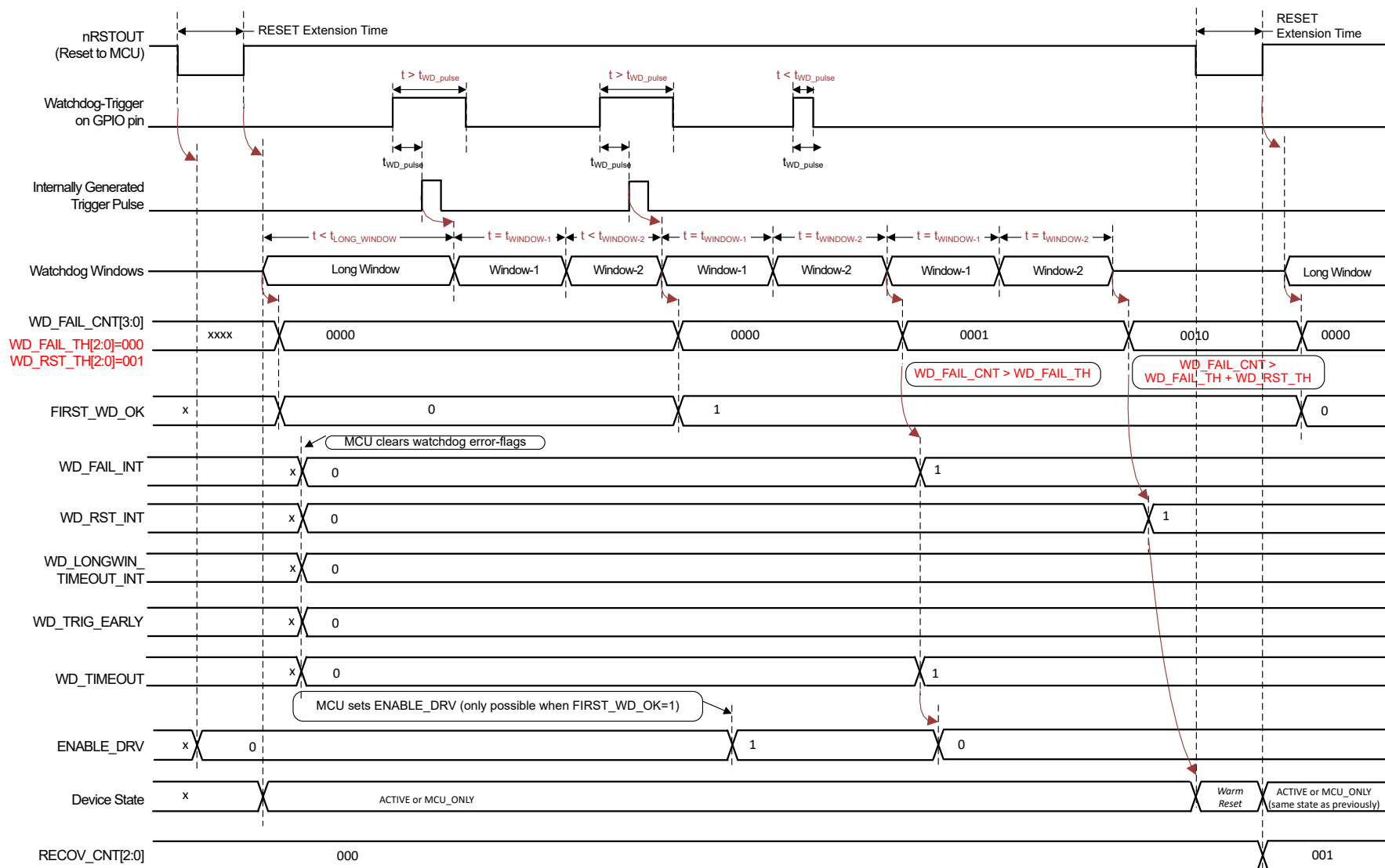
Figure 8-45. Watchdog in Trigger Mode – Bad Events (Too Short or no Trigger in Window-2) After Start-up
