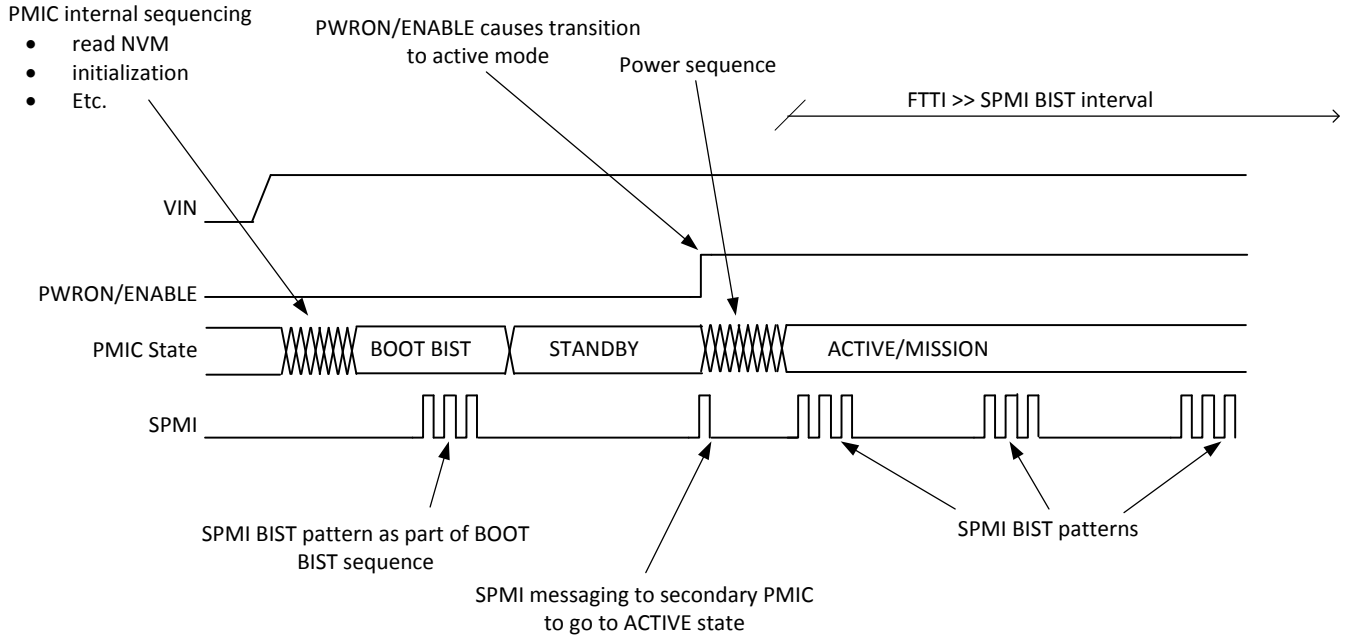
Figure 8-40. SPMI-BIST Operation
