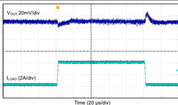
Figure 9-52. Load Transient Response, Auto Mode. 2.2 MHz Single Phase.
