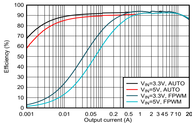
Figure 9-12. Efficiency in 2.2 MHz 4-Phase Mode
