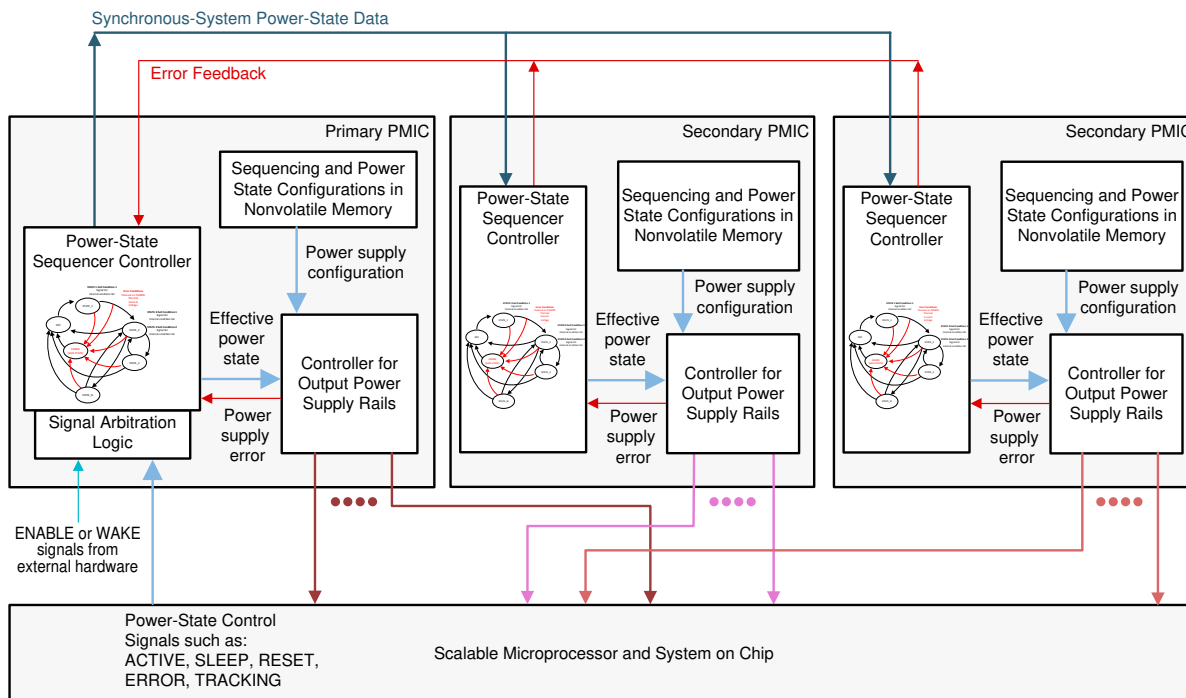
Figure 8-36. Multi-PMIC Power State Synchronization Block Diagram
