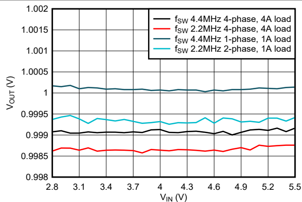
Figure 9-23. Line Regulation
