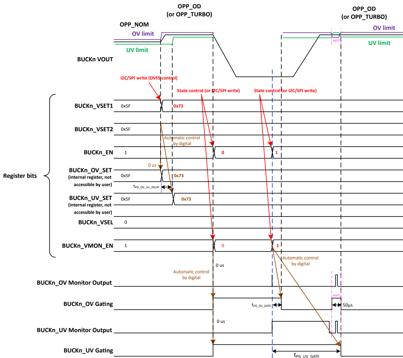
Figure 8-14. DVS Voltage and OV UV Threshold Level Change Timing Diagram
