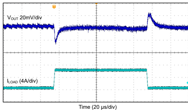
Figure 9-48. Load Transient Response, FPWM Mode. 4.4 MHz 3-Phase.
