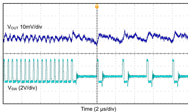
Figure 9-39. PWM to PFM Transition 2.2 MHz Single Phase Auto Mode
