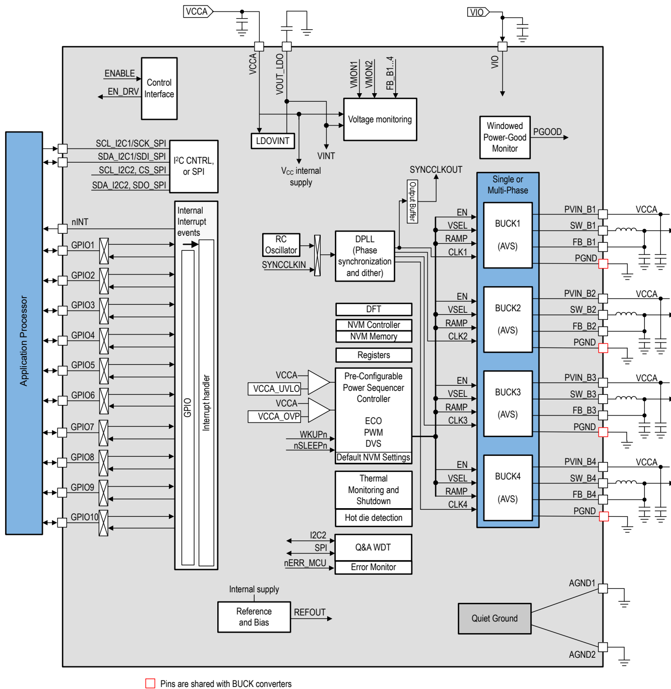
Figure 8-1. LP8764-Q1 Functional Block Diagram
