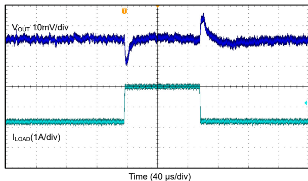
Figure 9-40. Load Transient Response, Auto Mode. 4.4 MHz Single Phase
