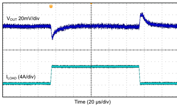
Figure 9-53. Load Transient Response, FPWM Mode. 2.2 MHz 3-Phase.
