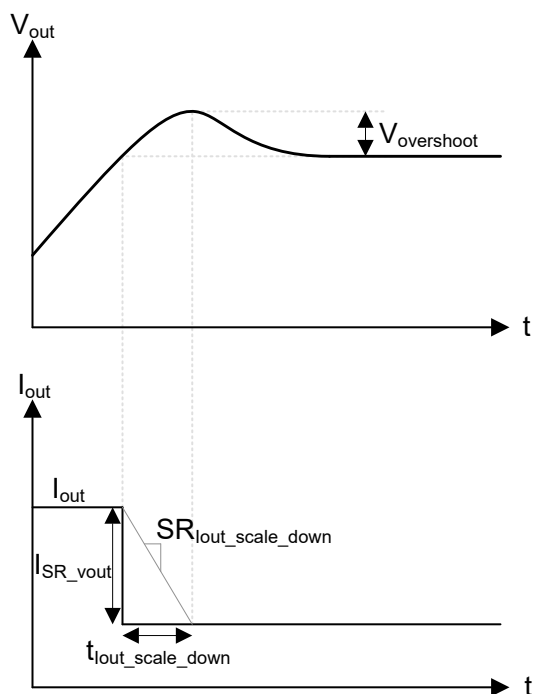
Figure 9-9. Overshoot
