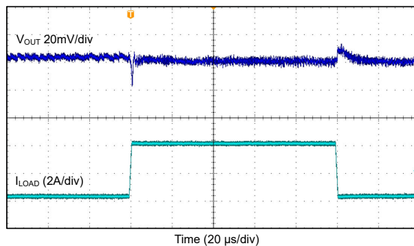
Figure 9-49. Load Transient Response, FPWM Mode. 4.4 MHz 2-Phase.
