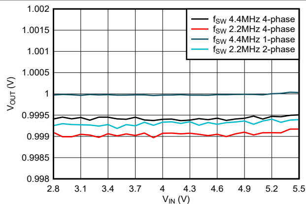
Figure 9-22. Line Regulation
