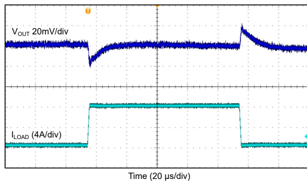
Figure 9-42. Load Transient Response, Auto Mode. 2.2 MHz 4-Phase.
