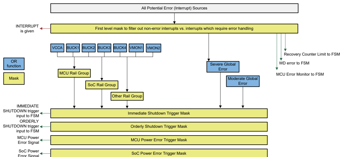
Figure 8-4. Error Source Hierarchical Mask System
