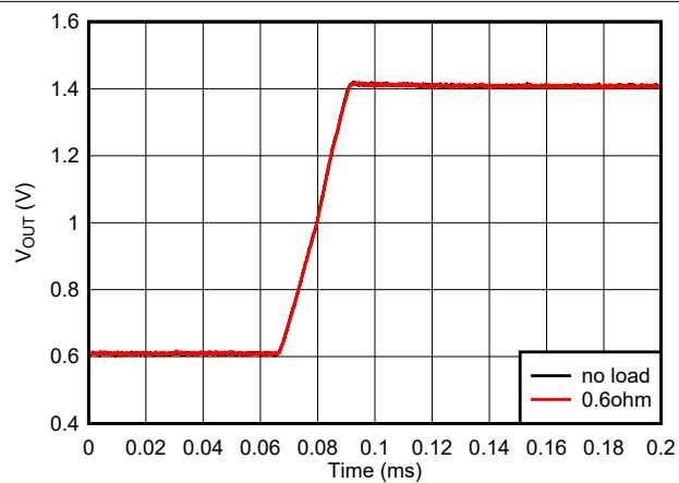
Figure 7-7. Buck Ramp-up Slew Rate
