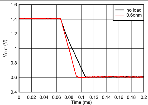
Figure 7-8. Buck Ramp-down Slew Rate
