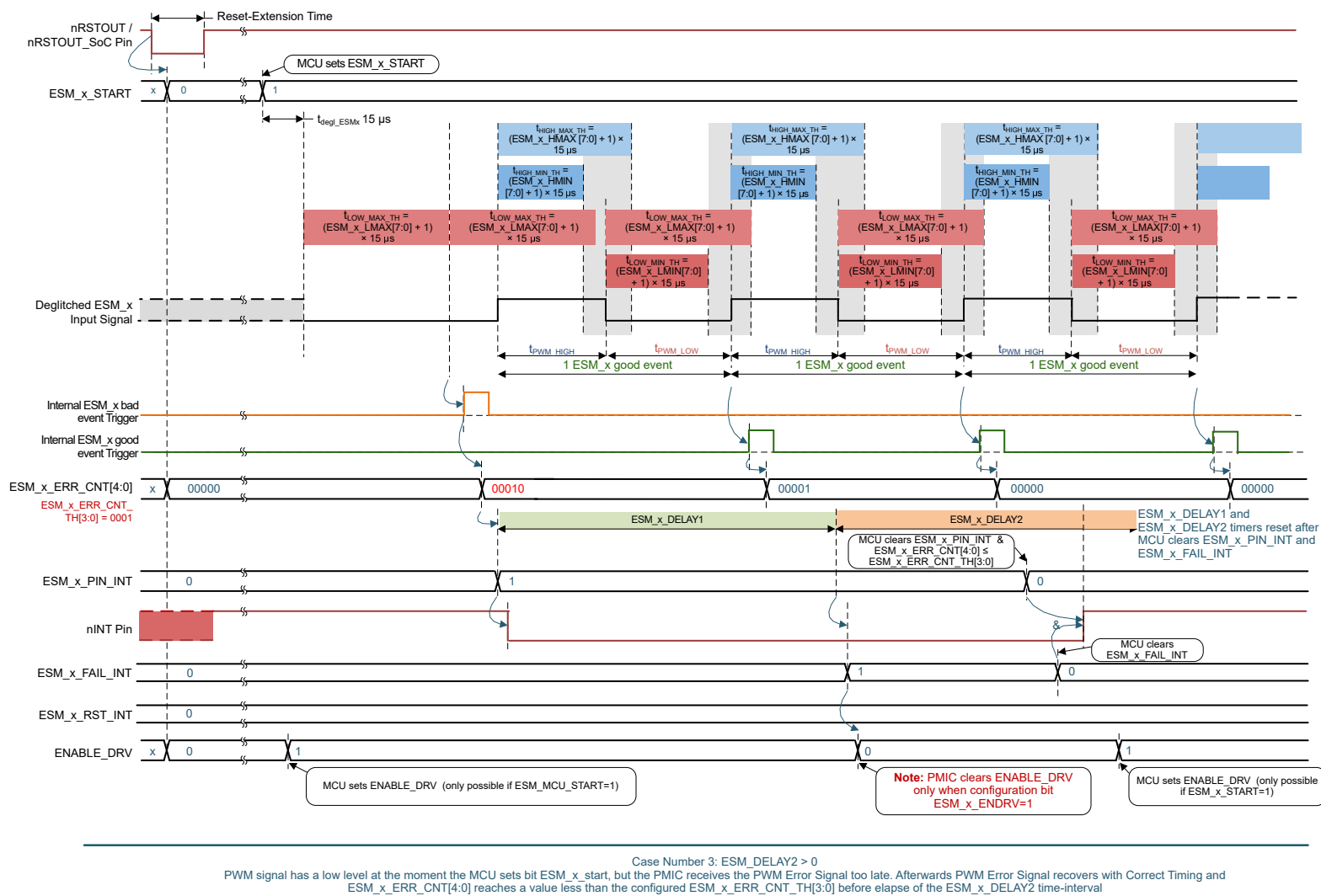
Figure 8-60. Example Waveform for ESM in PWM Mode – Case Number 3: ESM_MCU Starts with Low-Level at Deglitched Input Signal, but Receives Too Late a Correct PWM Signal Afterwards (The _x stand for _MCU )
