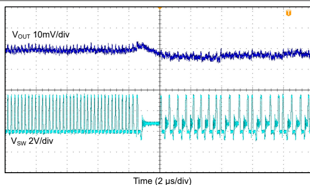
Figure 9-37. PWM to PFM Transition 4.4 MHz Single Phase Auto Mode
