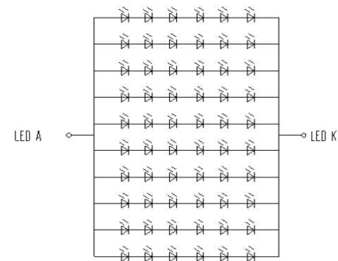
Backlight Circuit Diagram 6S-10P; If=100mA/LED
