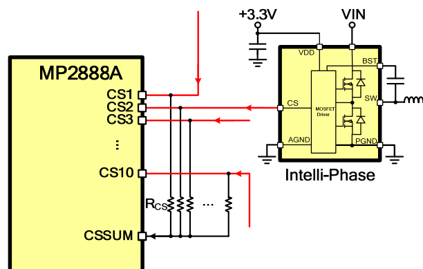
Figure 4: Phase Current Sense
