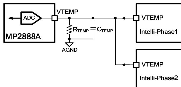
Figure 9: Temperature Sense for MP2888A with Intelli-Phase
