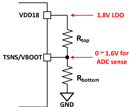
Figure 3: Circuit of Pin-Strap Boot Voltage
