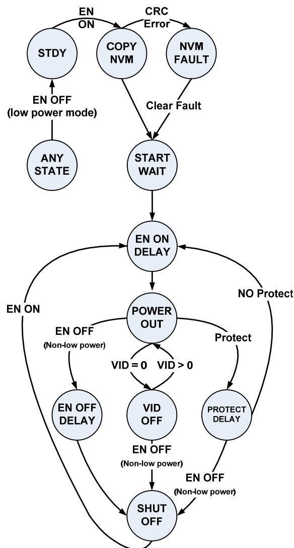
Figure 2: System State Machine
