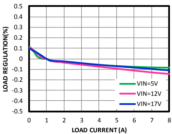
Load Regulation vs. Load Current
