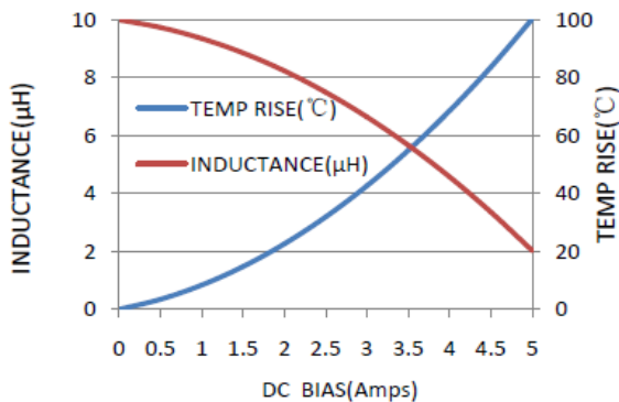
MWSA0518S-100MT
