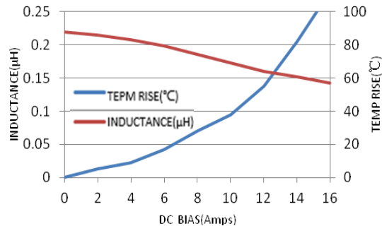
MWSA0402S-R22MT
