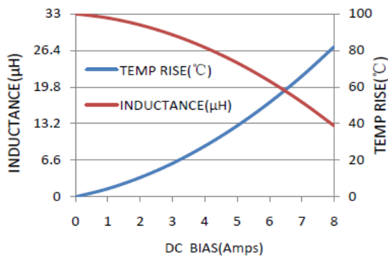
MWSA1004S-330MT
