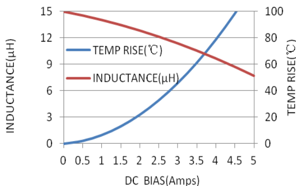
MWSA0624S-150MT
