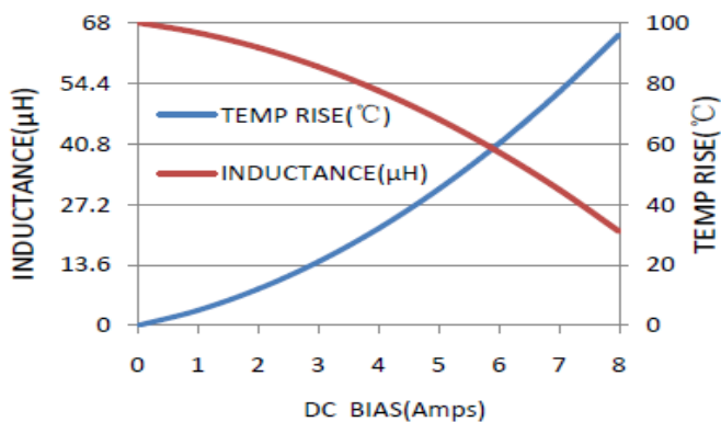
MWSA1206S-680MT
