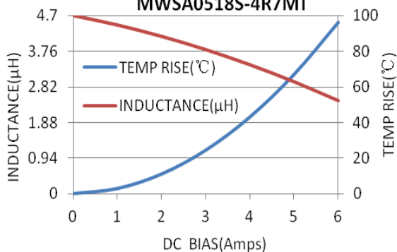
MWSA0518S-4R7MT
