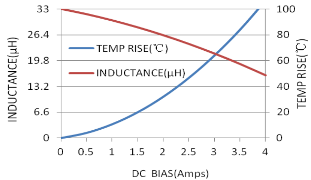
MWSA0603S-330MT
