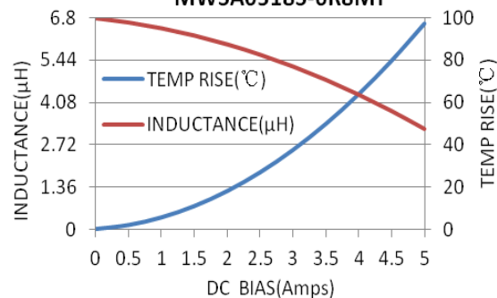
MWSA0518S-6R8MT
