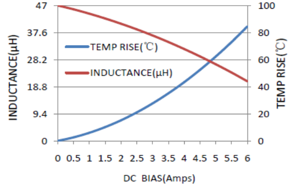
MWSA1004S-470MT
