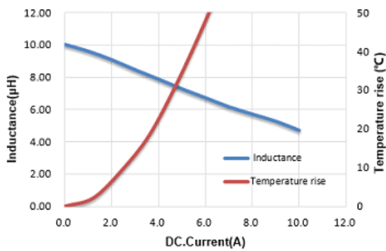
MWSA0603S-100MT
