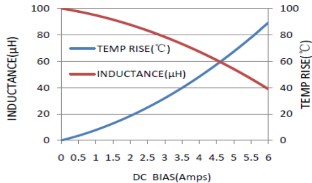
MWSA1206S-101MT
