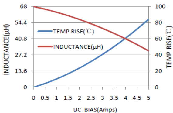
MWSA1004S-680MT
