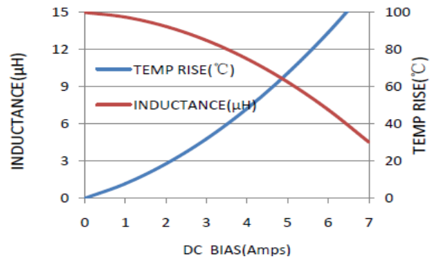
MWSA0603S-150MT
