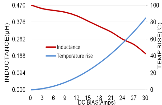
MWSA0603S-R47MT
