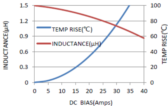
MWSA1204S-1R5MT
