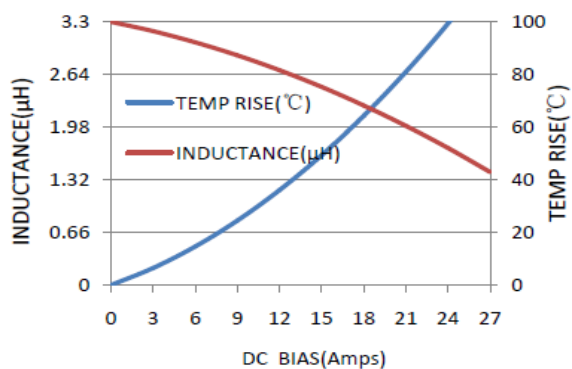
MWSA1004S-3R3MT
