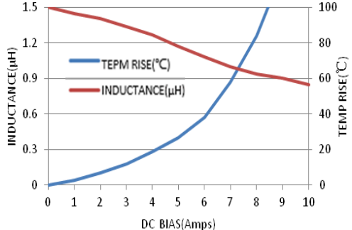
MWSA0402S-1R5MT
