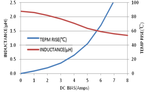
MWSA0402S-2R2MT
