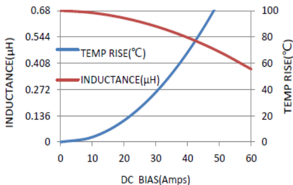
MWSA1204S-1R0MT
