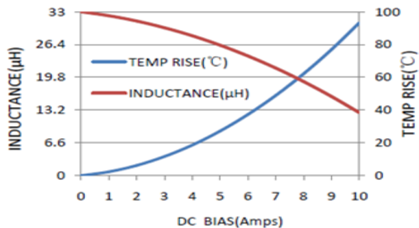
MWSA1206S-330MT
