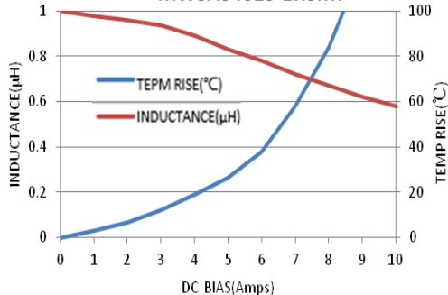
MWSA0402S-1R5MT
