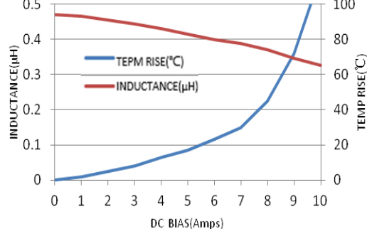
MWSA0402S-R68MT
