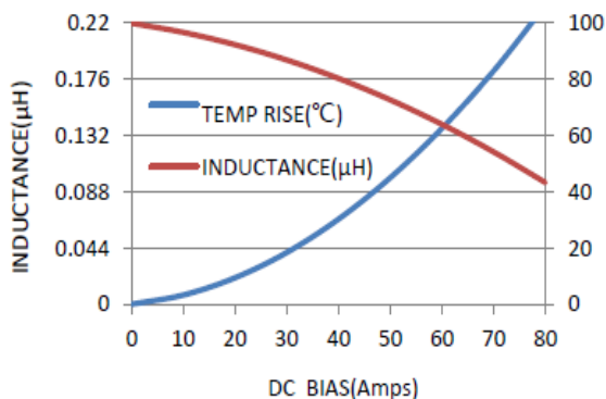
MWSA1204S-R68MT
