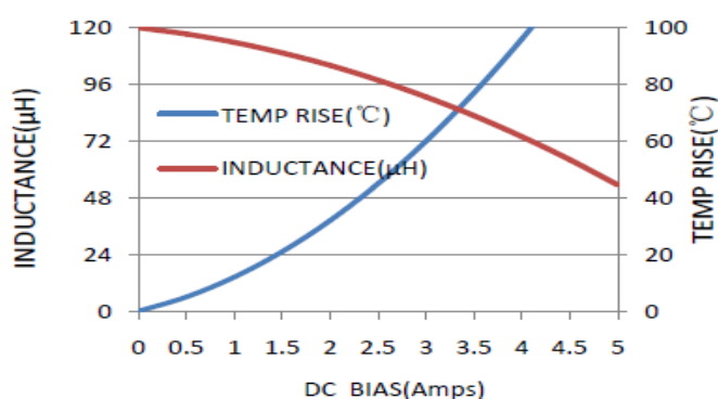
MWSA1206S-121MT
