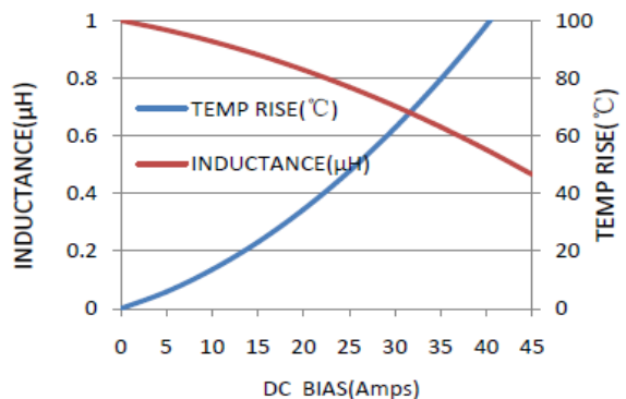
MWSA1004S-2R2MT
