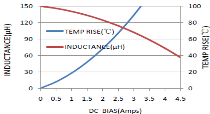
MWSA1206S-151MT
