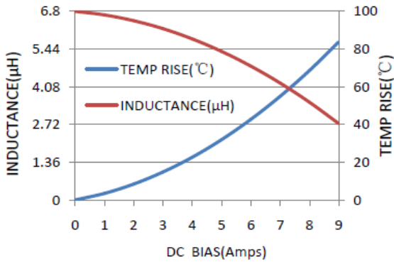
MWSA0603S-100MT
