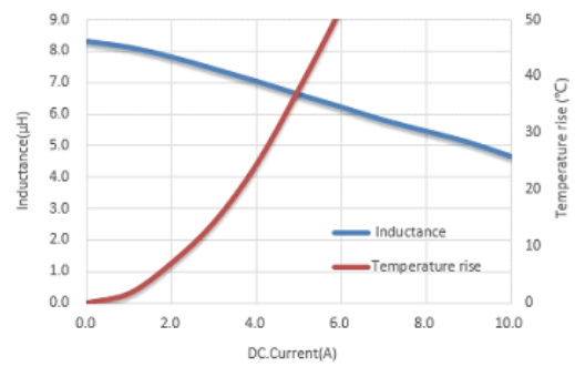
MWSA0603S-8R2MT
