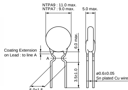
NTPA7/NTPA9 Series
