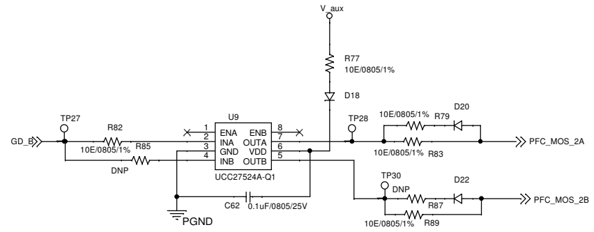
PFC Driver 2
