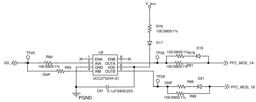
PFC Driver 1
