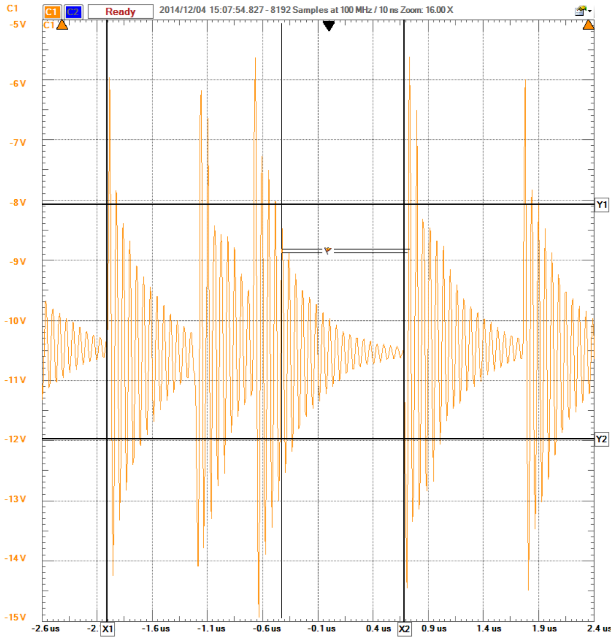
V_{out} node high frequency capture
