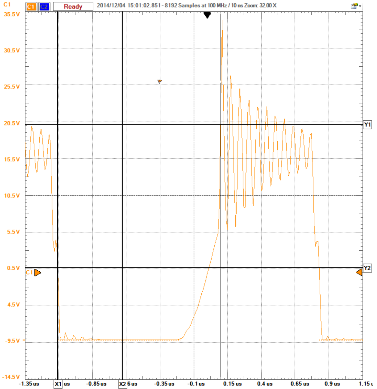
Close up of single cycle on Phase node
