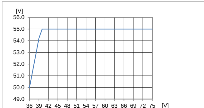
Max adjustable output voltage vs. input voltage at T_{P1} = +25^{\circ}\text{C} .
