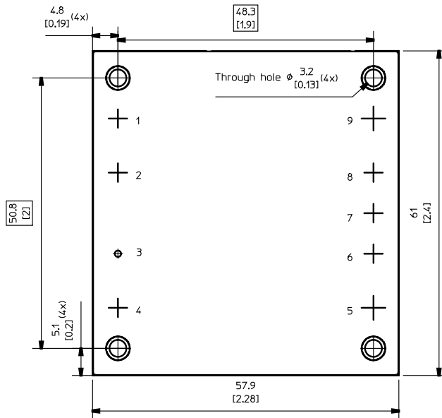
RECOMMENDED FOOTPRINT - TOP VIEW
