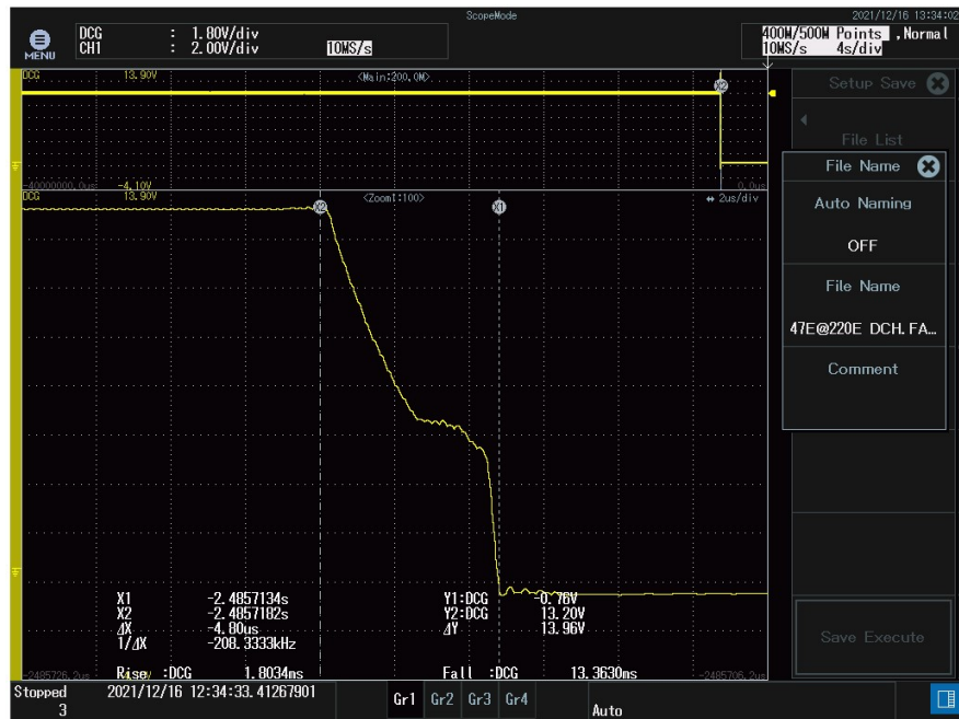
Gate Discharge waveform of Main Discharge MOSFET
