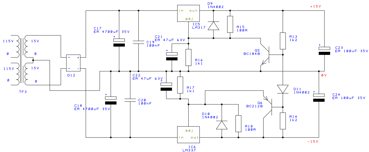
DUAL RAIL PSU Mutual Shutdown Circuitry
