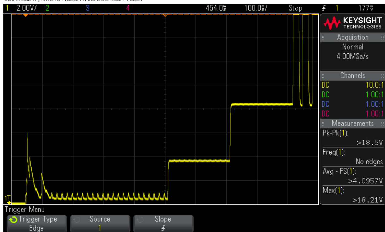
Figure 1: Phihong AT, model no. POE29U-1AT(PL), zoomed in
