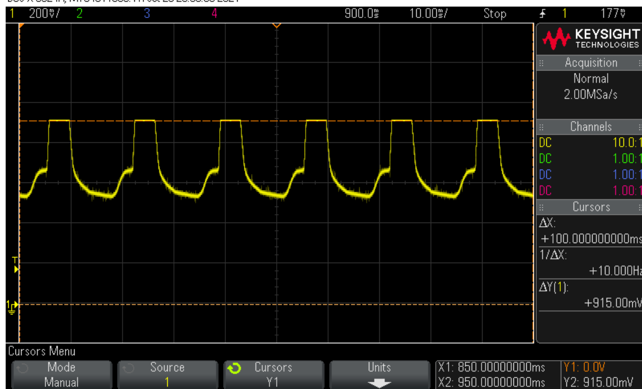
Figure 6: Zoomed in waveform of the delay before the detection
