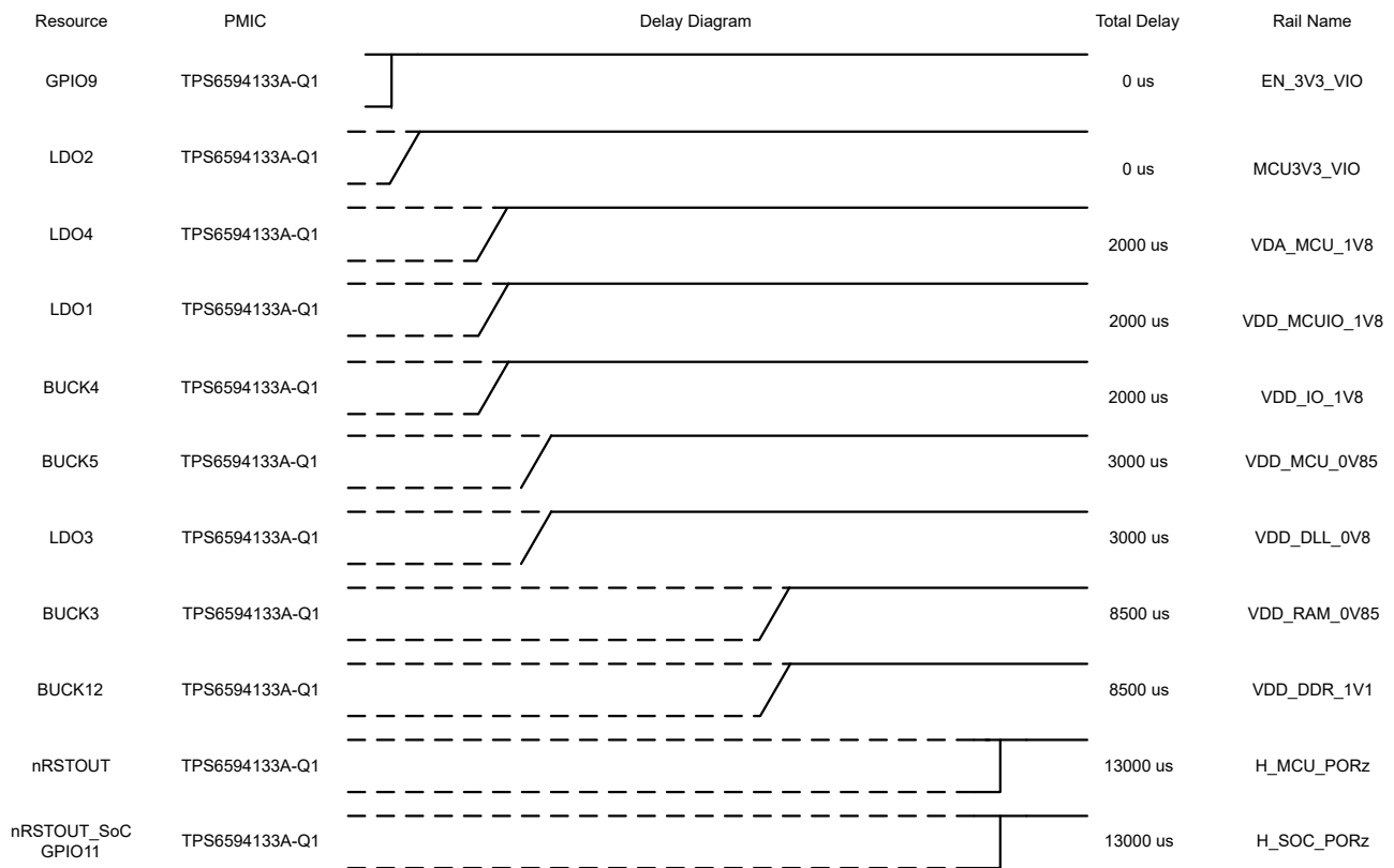
Figure 5-11. TO_ACTIVE Sequence
