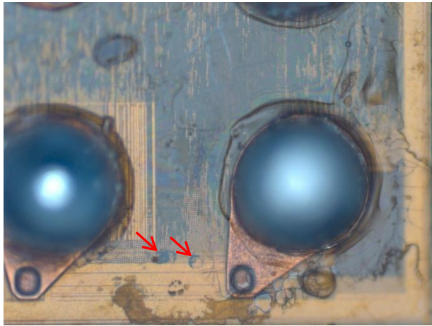
Figure 1. Optical pictures of package surface
