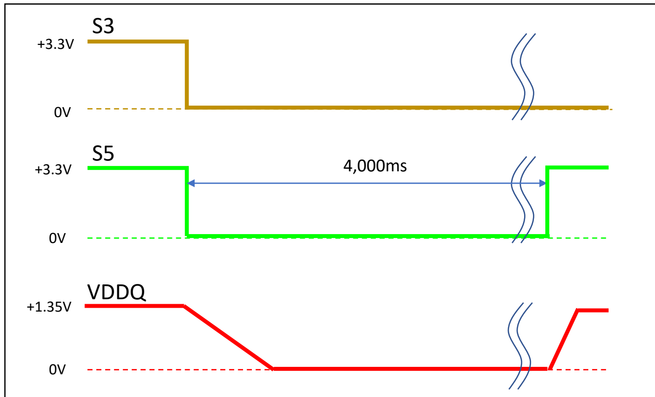
Waveform (B)
