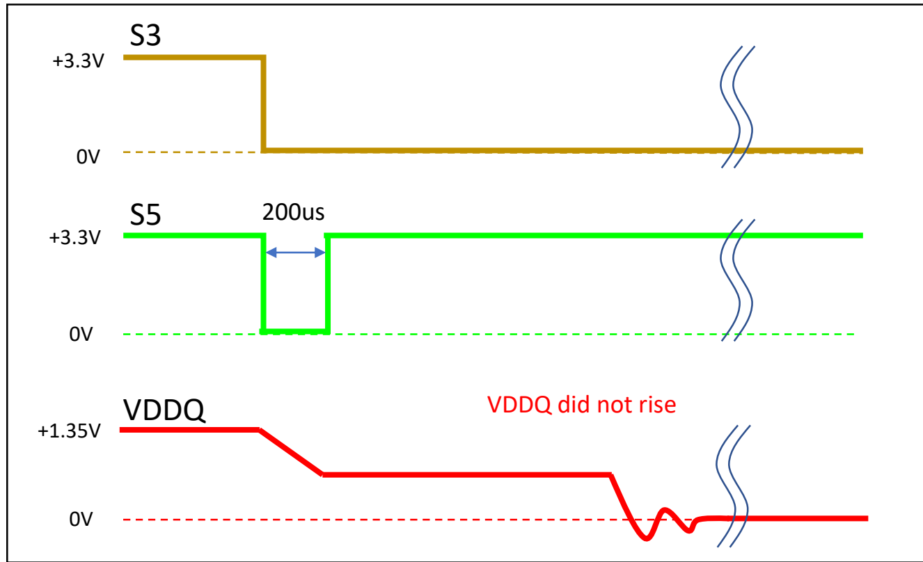
Waveform (A)
