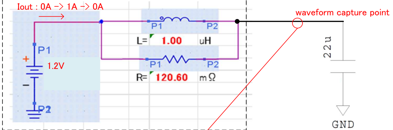
TPSM82903 pseudo circuit
