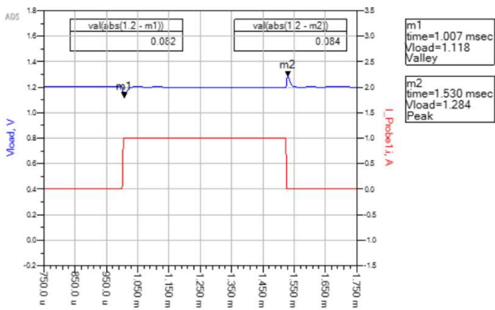
Captured waveform at above point
