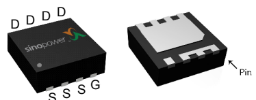
DFN3x3D-8_EP
