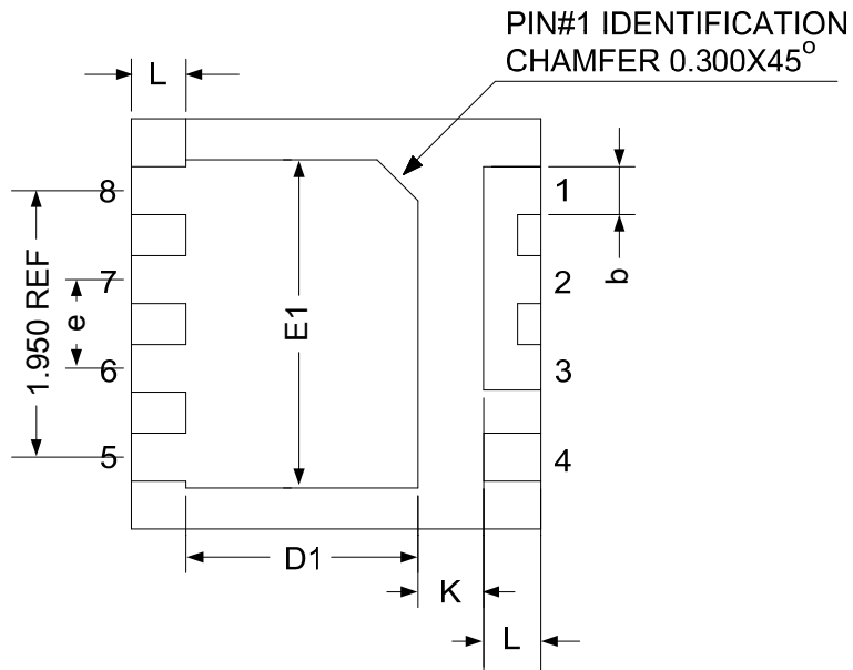
Bottom View
