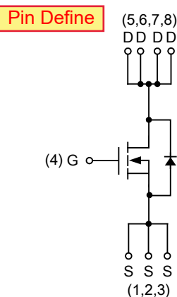
N-Channel MOSFET
