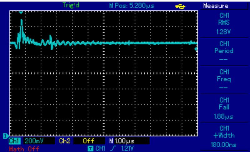
FB_without_load_40v_2
