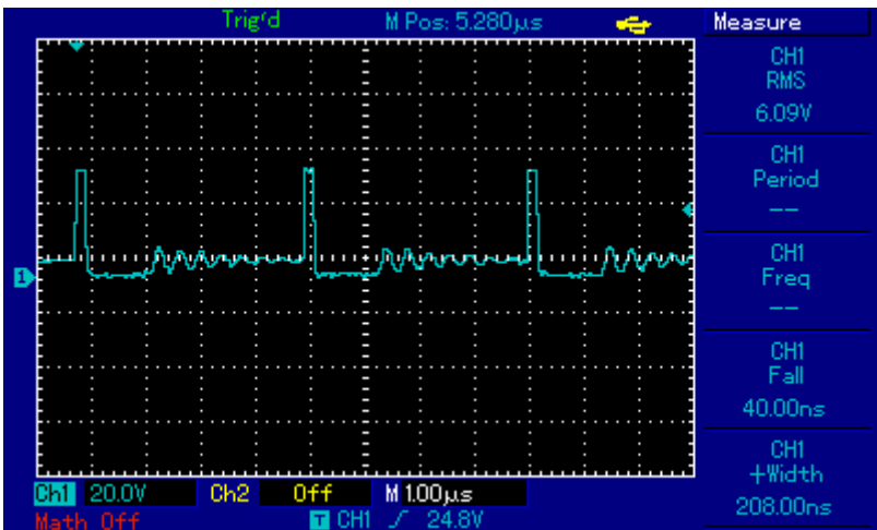
SW_with_load_40v_1
