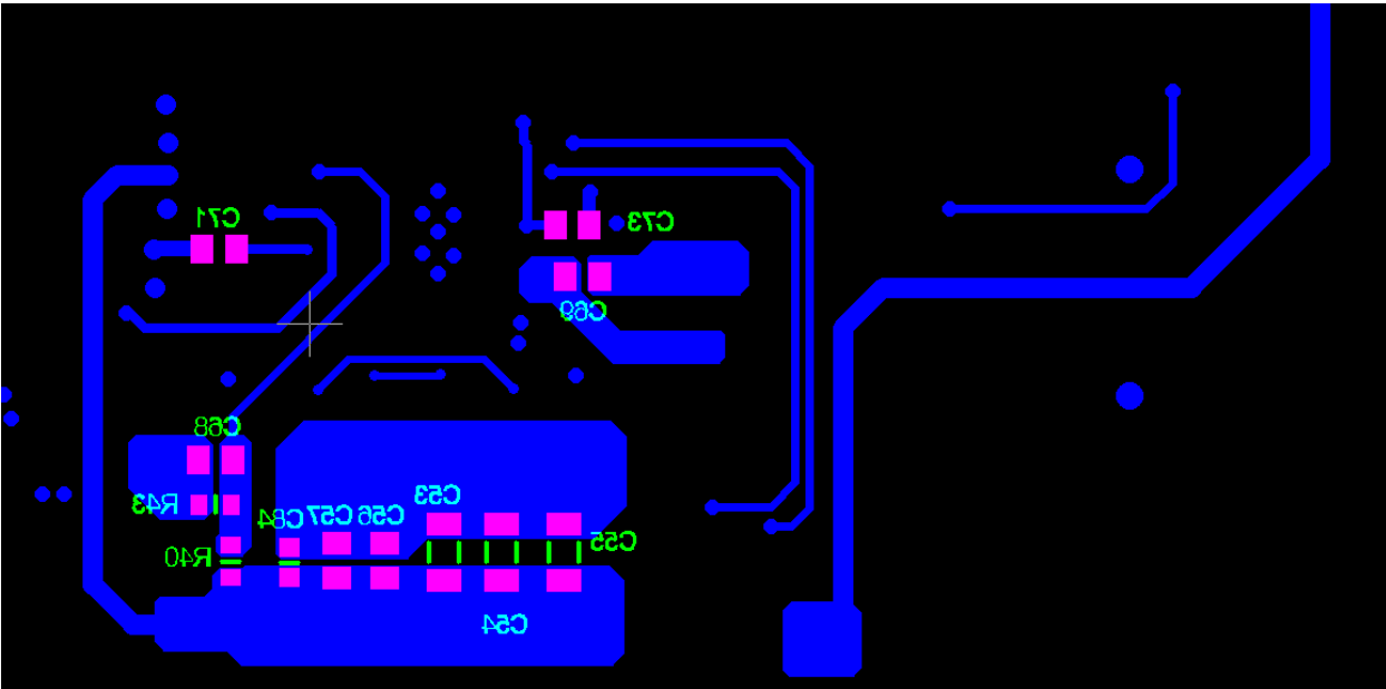
close view of bottom side layer and component.
