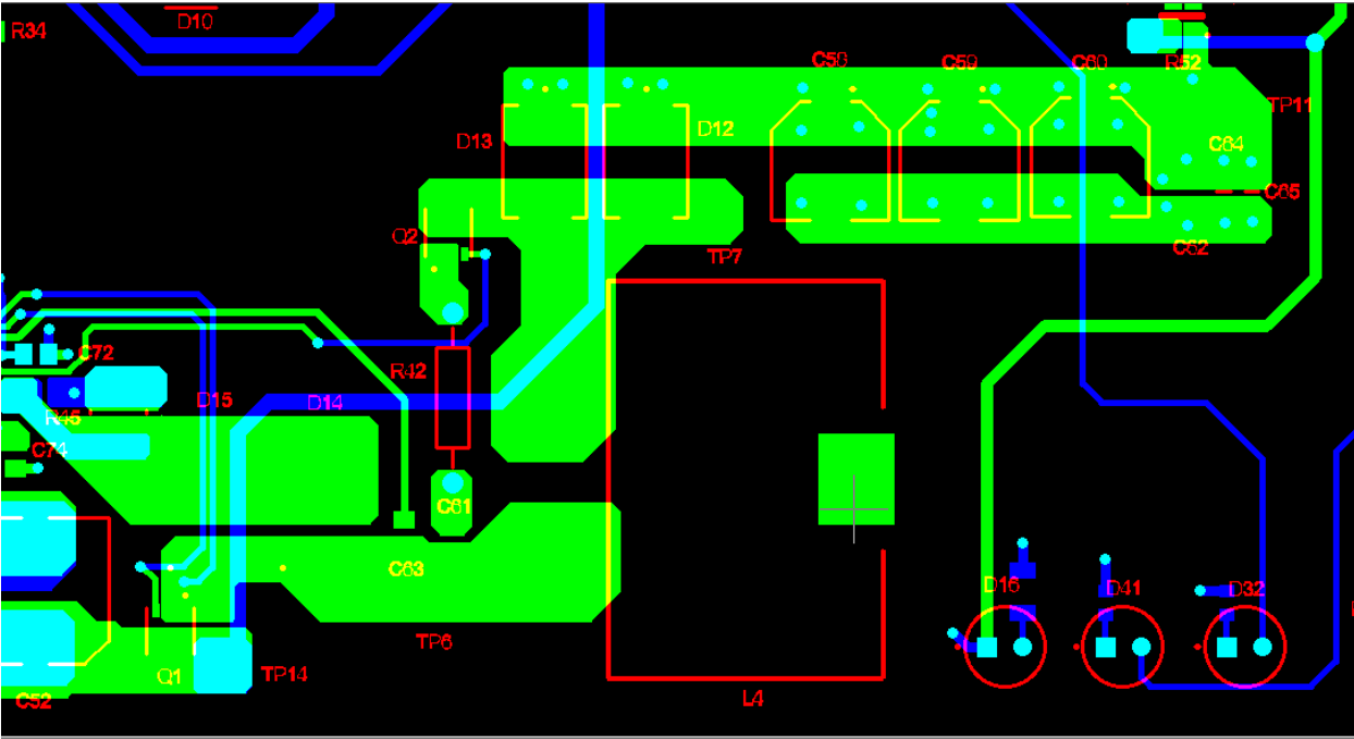
Close view of top and bottom side layer of inductor, output diodes and capacitors.
