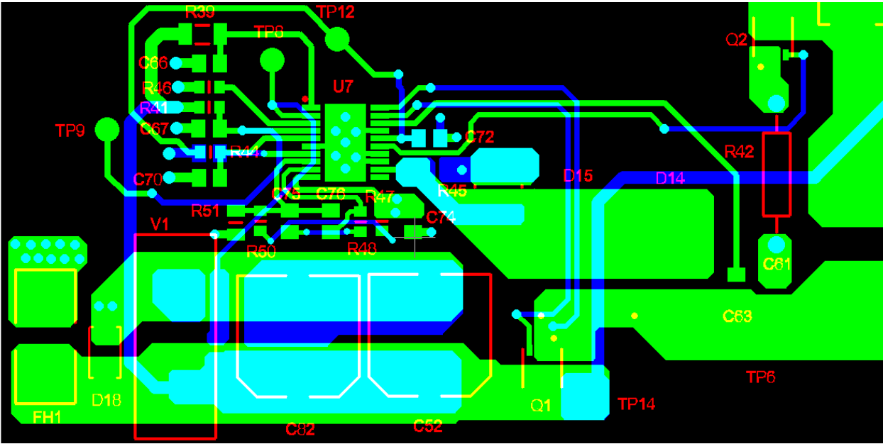
Close view of top and bottom layer of input capacitors, IC LM5118 and components.
