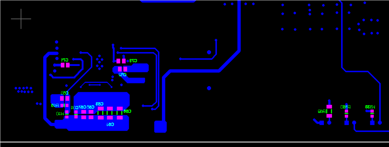
Bottom side layer.
