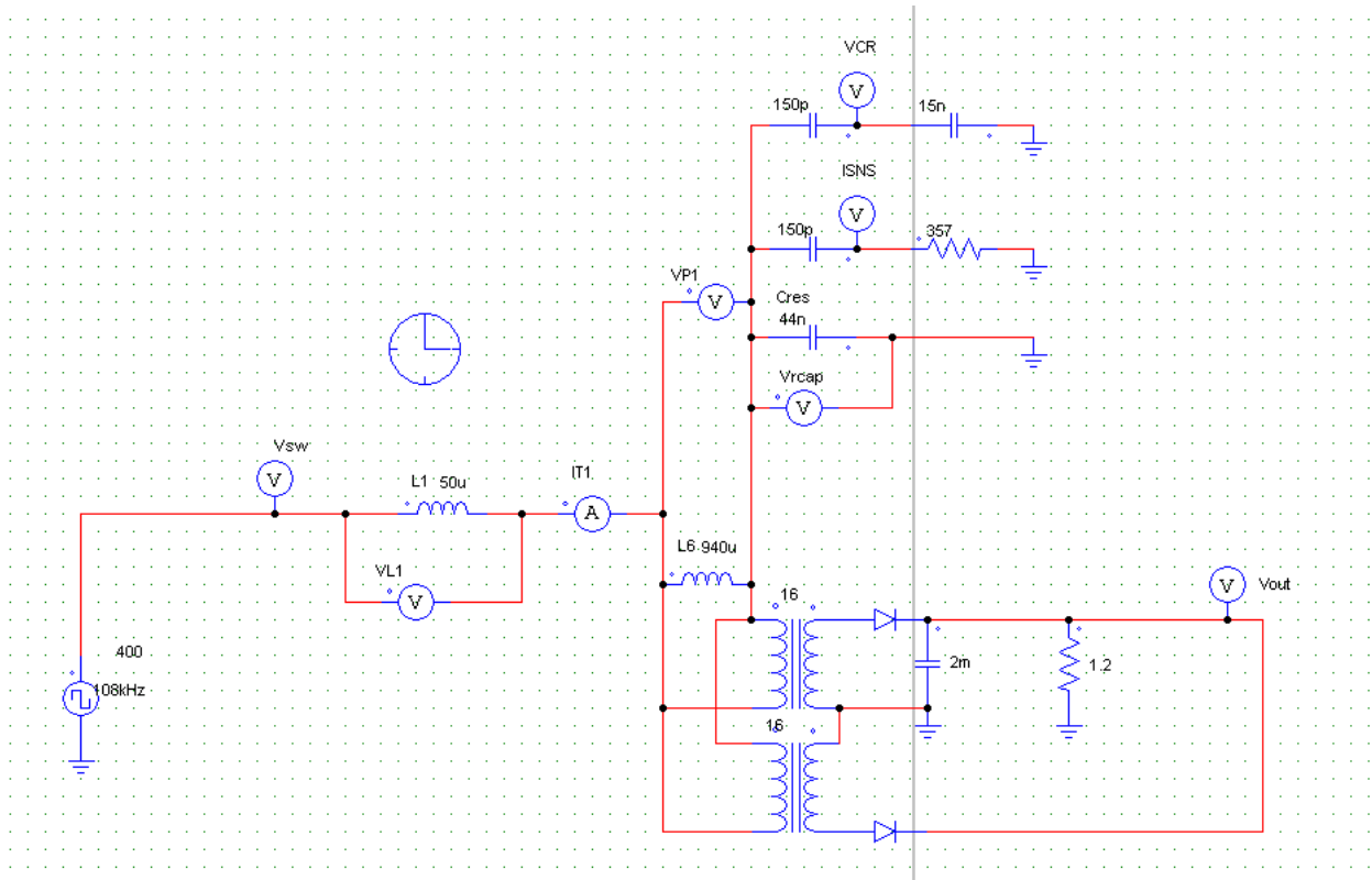
VCR ISNS and IT1 at resonant frequency of 108 kHz
