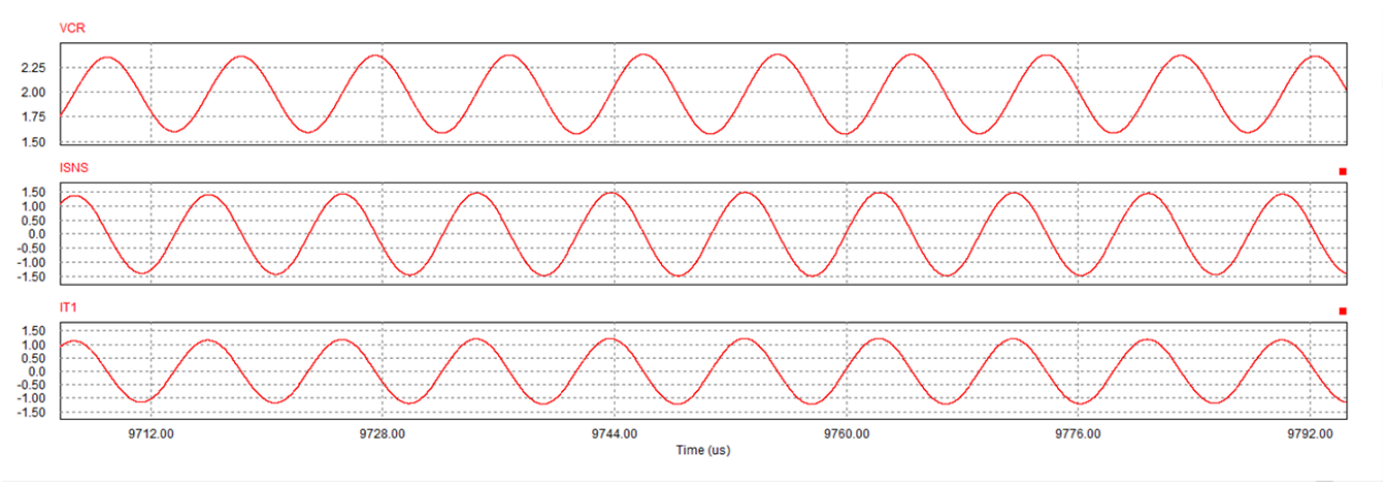
VCR ISNS and IT1 at resonant frequency of 108 kHz
