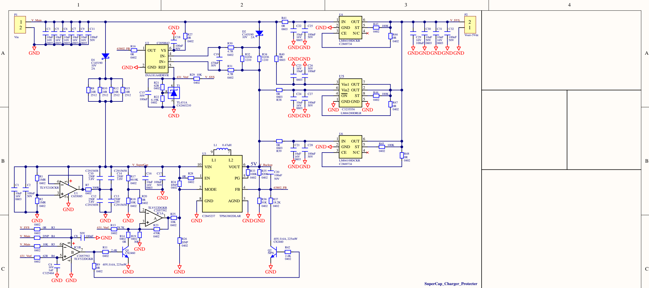
SuperCap_Charger_Protector
