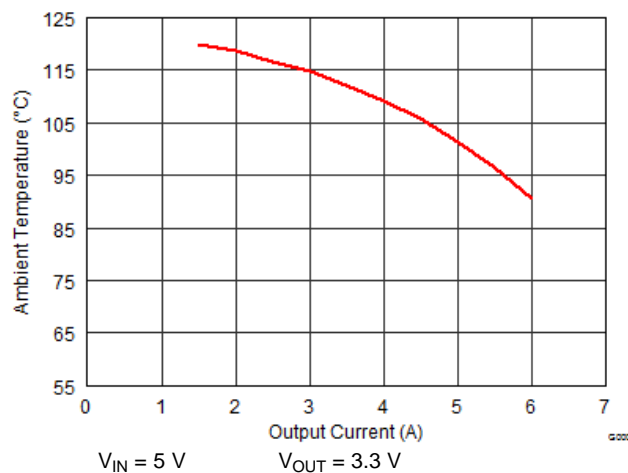
Figure 36. Maximum Ambient Temperature for T j =125°C (TPSM82480 EVM)
