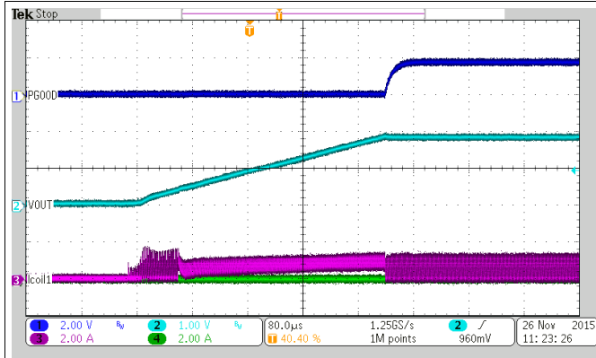
Figure 22. Startup into 3.3 \Omega resistor
