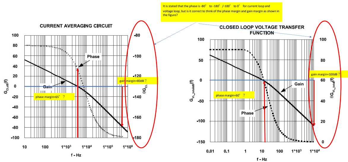
Figure 30. Bode Plot of the Current Averaging Circuit.
