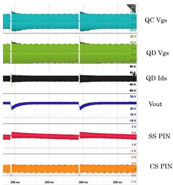
Fig.1 Start up operation
