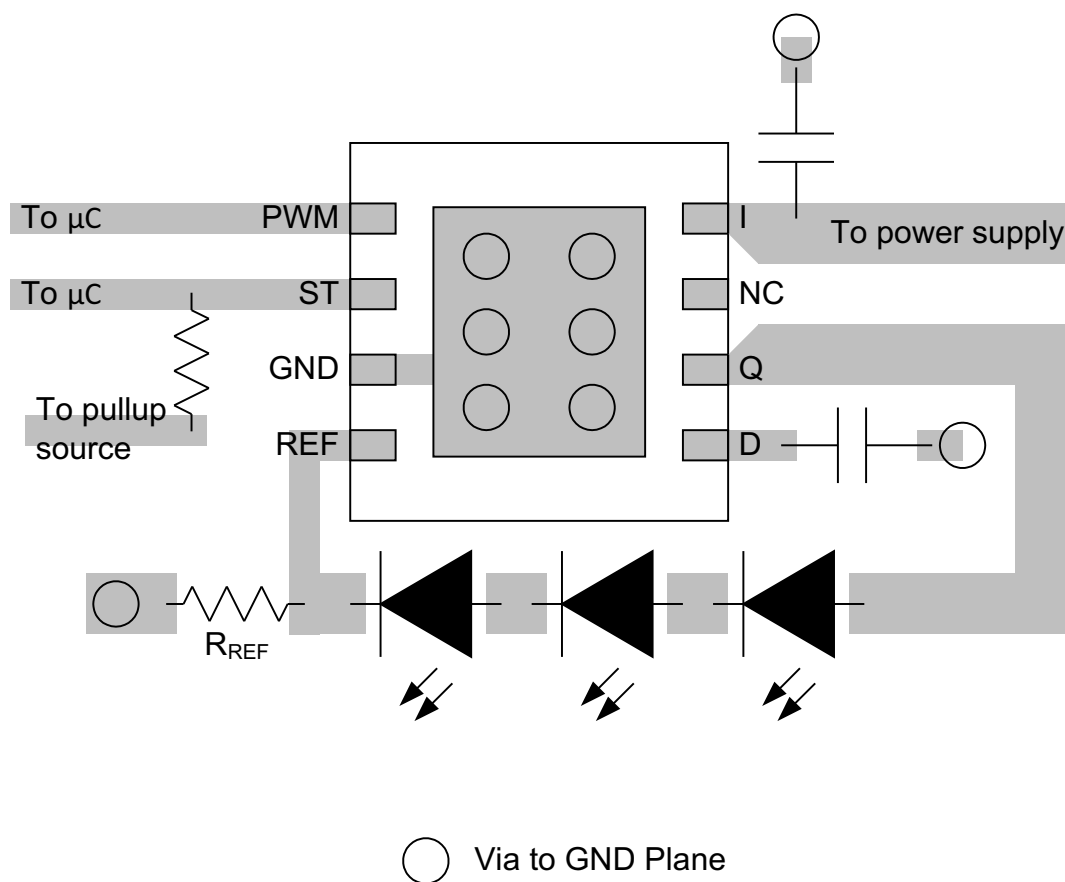
Figure 8. PCB Layout
