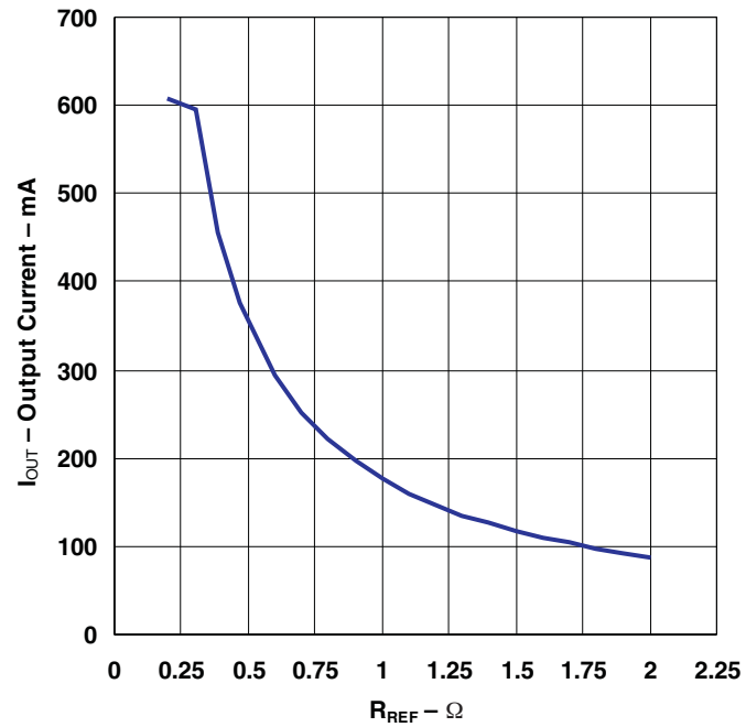
Figure 7. Output Current vs External Resistor
