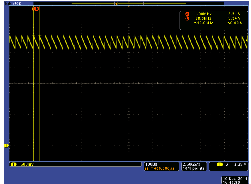
Sample B Oscillation frequency : 40kHz
