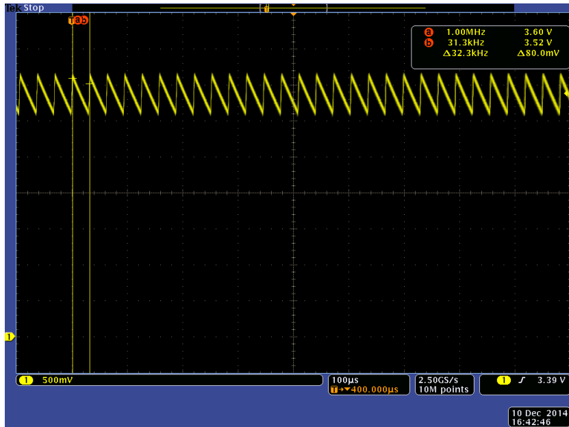
Sample A Oscillation frequency : 32.3kHz
