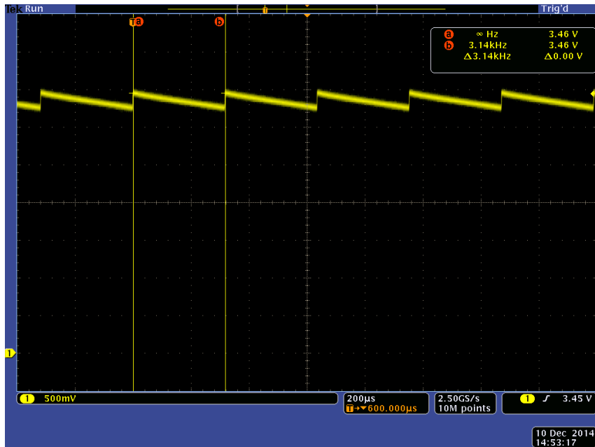
Sample A Oscillation frequency : 3.14kHz
