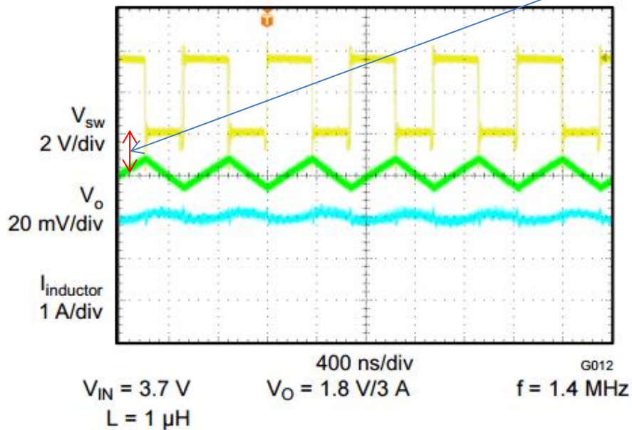
Figure 12. PWM Operation
