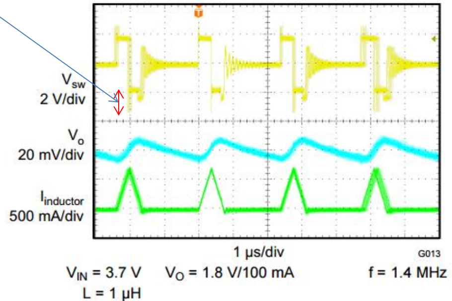
Figure 13. PFM Operation
