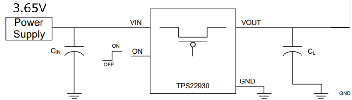
Simplified Schematic
