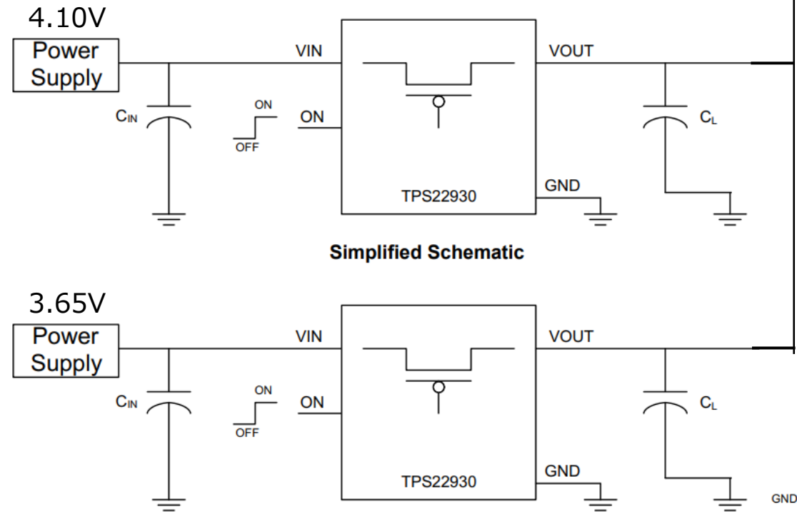
Simplified Schematic
