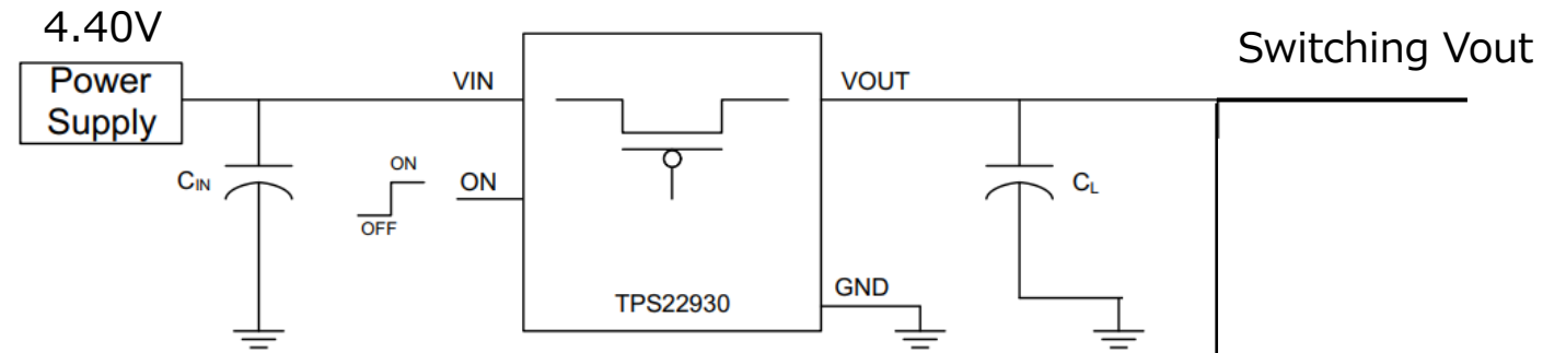
Simplified Schematic
