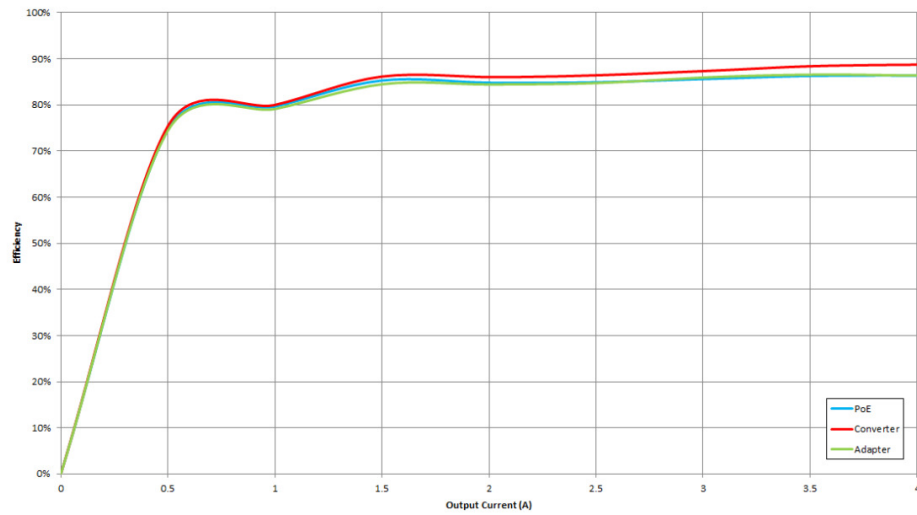
Figure 6. Efficiency of the TPS2373-3EVM-024, V_{IN} = 48\text{ V}
