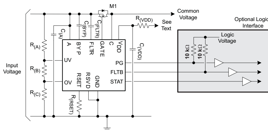
Figure 21. Design Template
