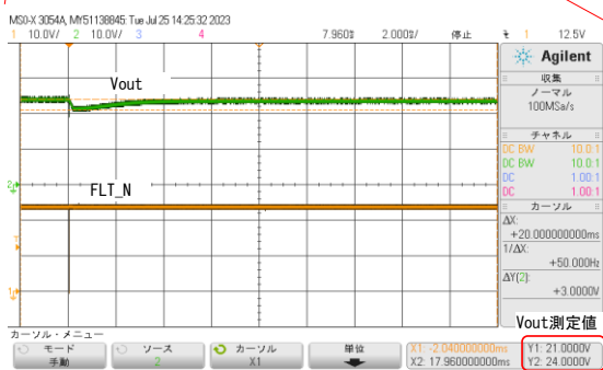
TPS26631 during load change from 20ohm to 9ohm
