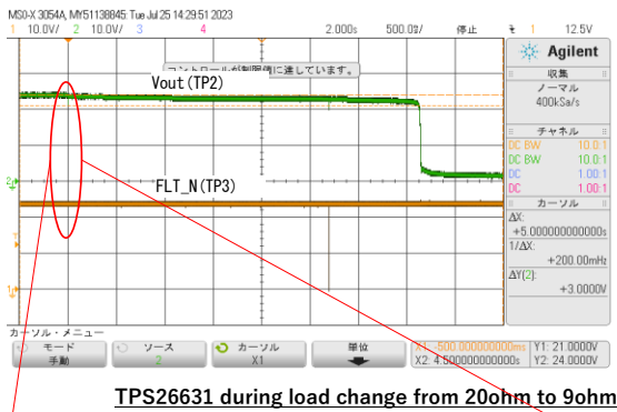
TPS26631 during load change from 20ohm to 9ohm
