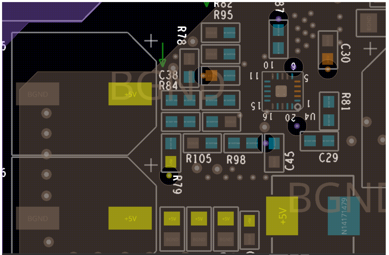
Inner layer 1 Ground plane
