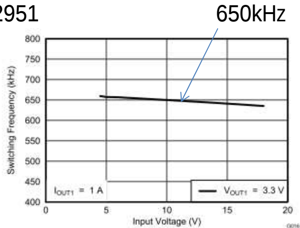
Figure 16. VO1 = 3.3V, SW-frequency vs Input Voltage (PWP)
