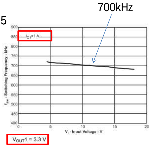
Figure 12. Switching Frequency vs Input Voltage
