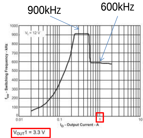
Figure 14. Switching Frequency vs Output Current
